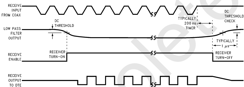
FIGURE 2. Receiver Timing
