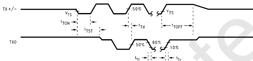
FIGURE 9. Transmitter Timing
