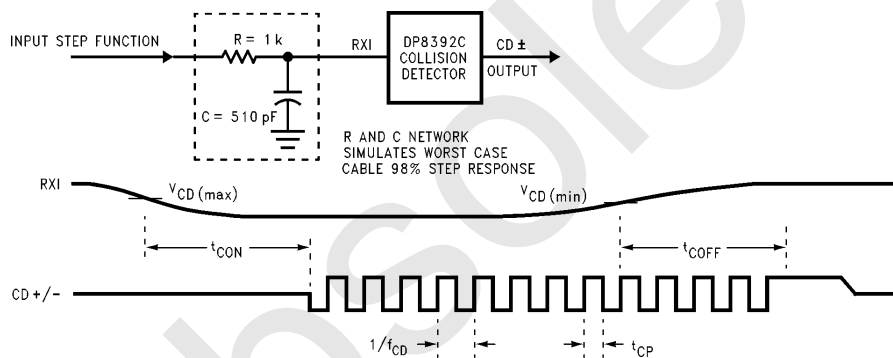
FIGURE 10. Collision Timing
