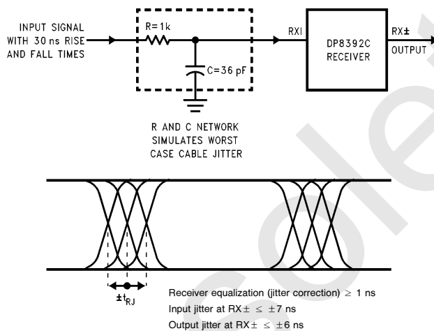
FIGURE 13. Receive Jitter Timing
