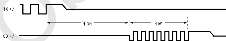
FIGURE 11. Heartbeat Timing
