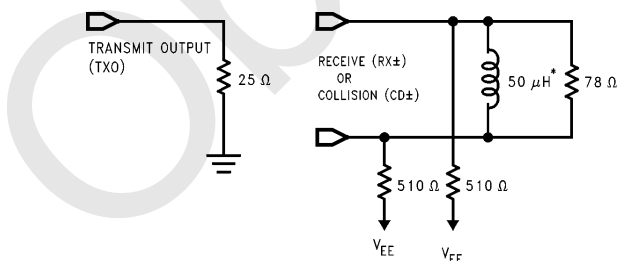
FIGURE 14. Test Loads
