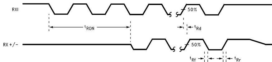
FIGURE 8. Receiver Timing
