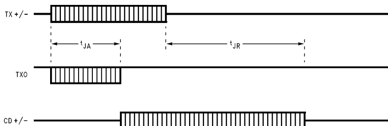
FIGURE 12. Jabber Timing
