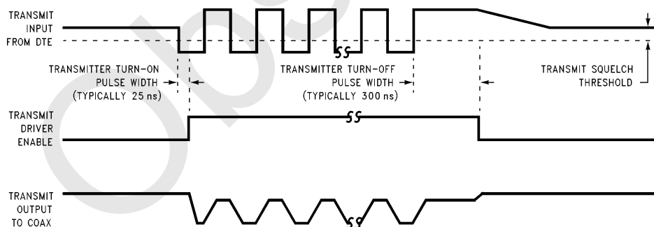
FIGURE 3. Transmitter Timing
