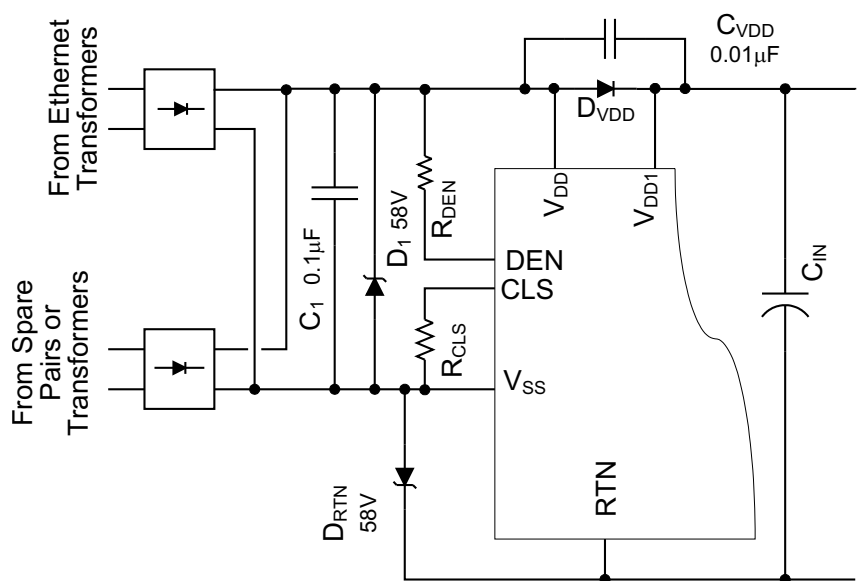
Figure 23. Additional Protection Against ESD
