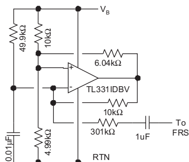
Figure 24. Frequency Dithering
