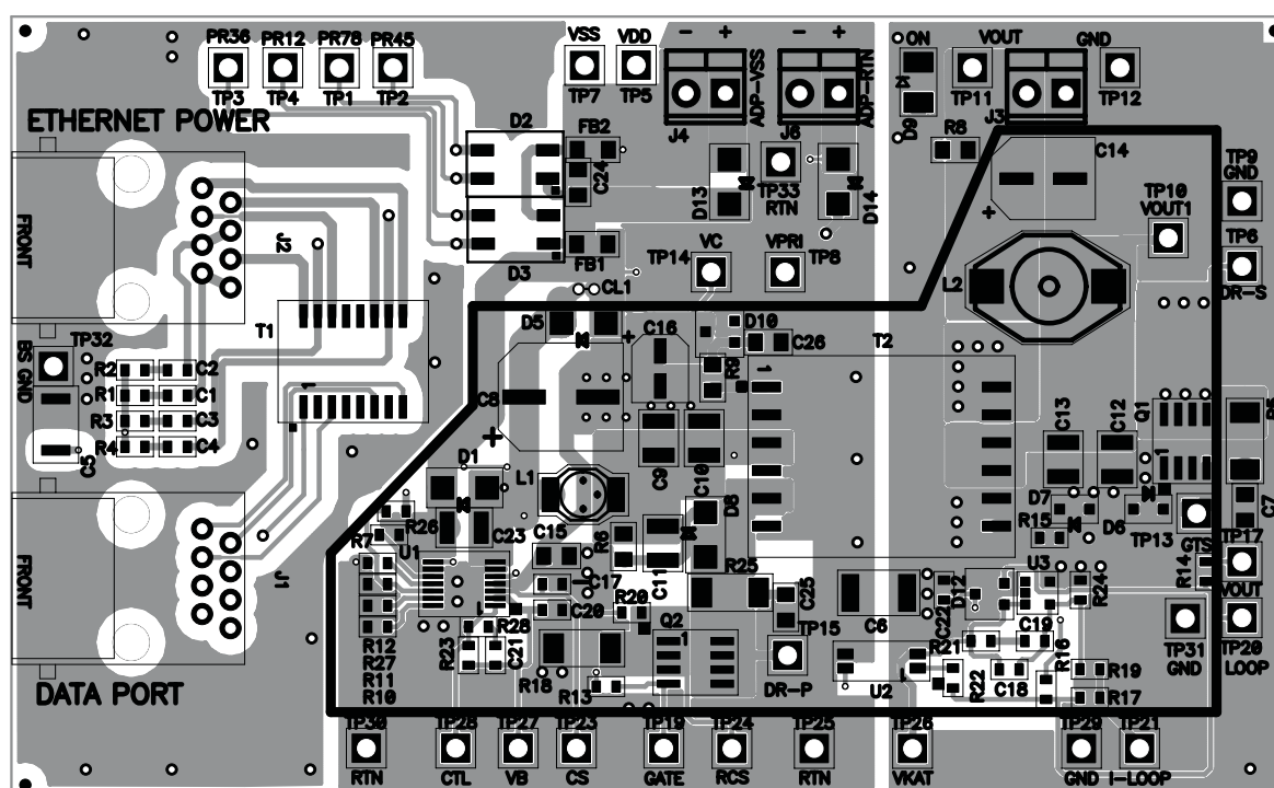
Figure 28. Top-Side Placement
