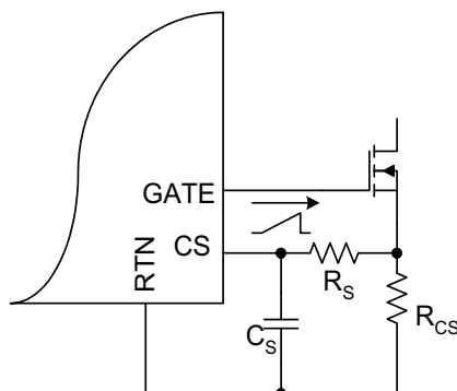
Figure 20. Additional Slope Compensation
