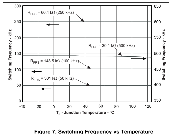
Figure 7. Switching Frequency vs Temperature
