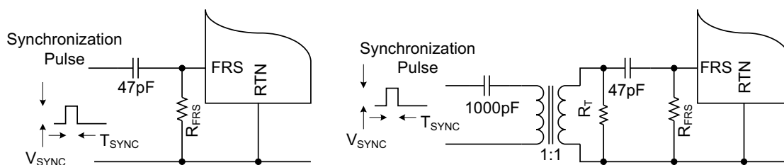
Figure 21. Synchronization
