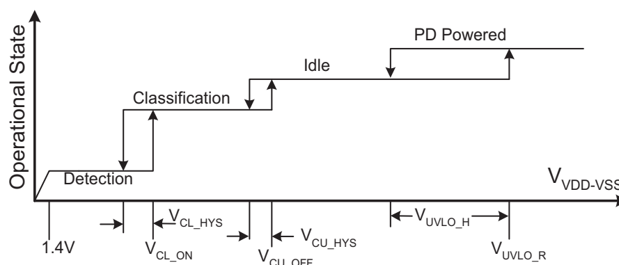
Figure 15. Threshold Voltages
