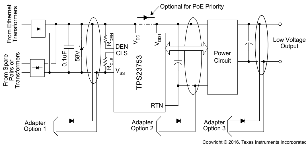
Figure 22. ORing Configurations
