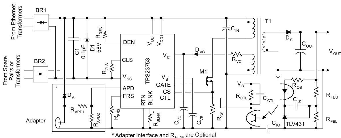
Figure 25. Basic TPS23753A Implementation
