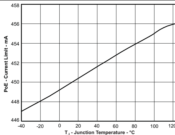
Figure 2. PoE Current Limit vs Temperature
