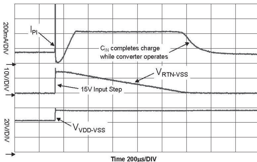
Figure 18. Response to PSE Step Voltage
