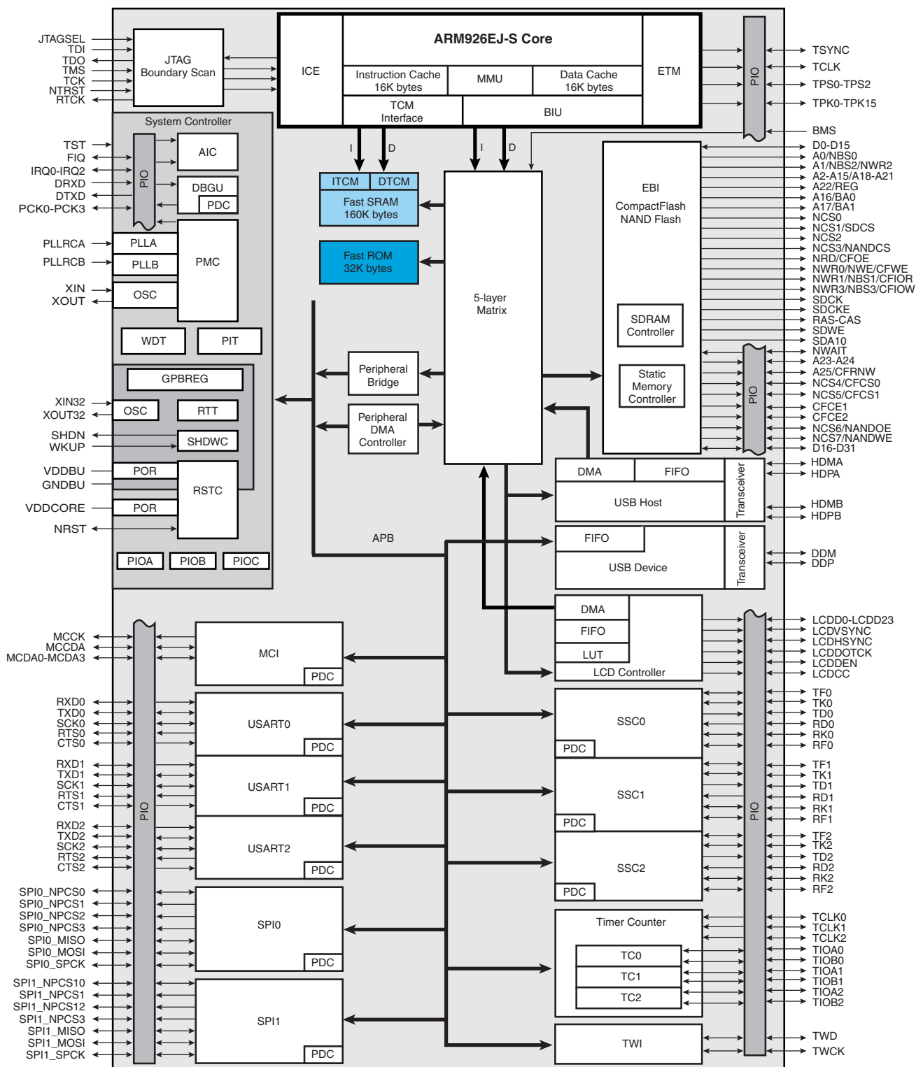
Figure 3-1. Block Diagram
