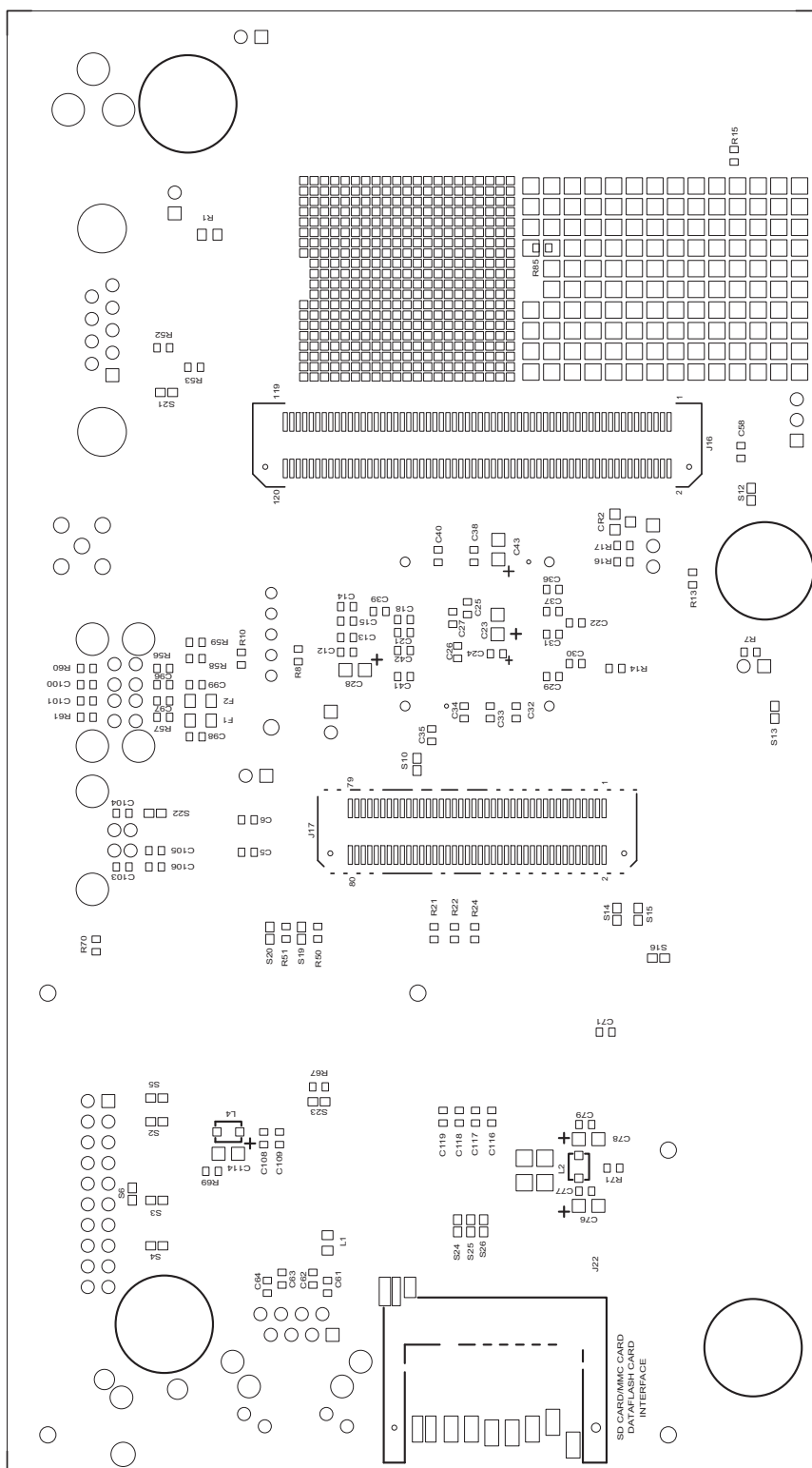
Figure 2-2. AT91SAM9G10-EK Layout - Bottom View
