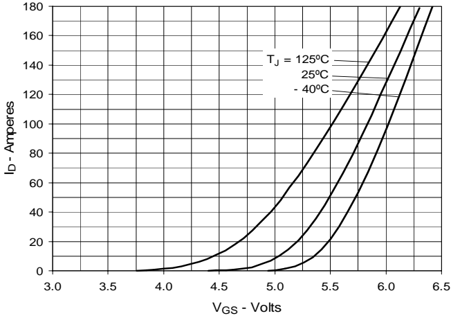
Fig. 7. Input Admittance
