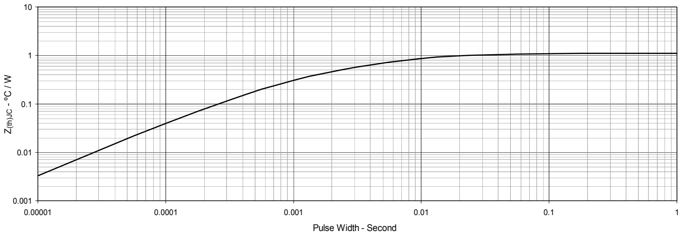
Fig. 22. Maximum Transient Thermal Impedance for Diode
