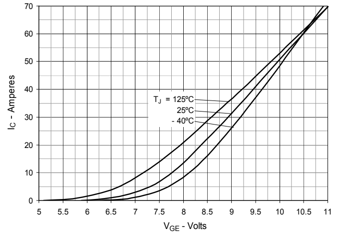
Fig. 6. Input Admittance
