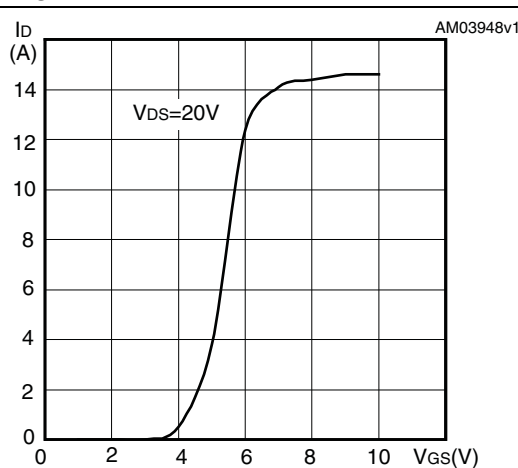
Figure 9. Transfer characteristics
