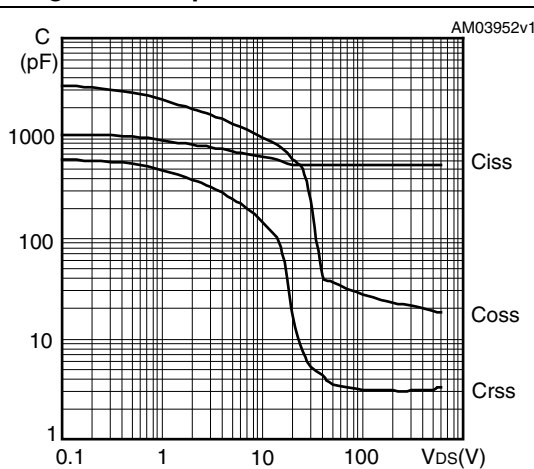
Figure 13. Capacitance variations
