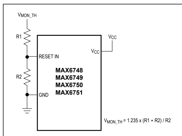
Figure 2. Calculating the Monitored Threshold Voltage ( V_{MON\_TH} )
