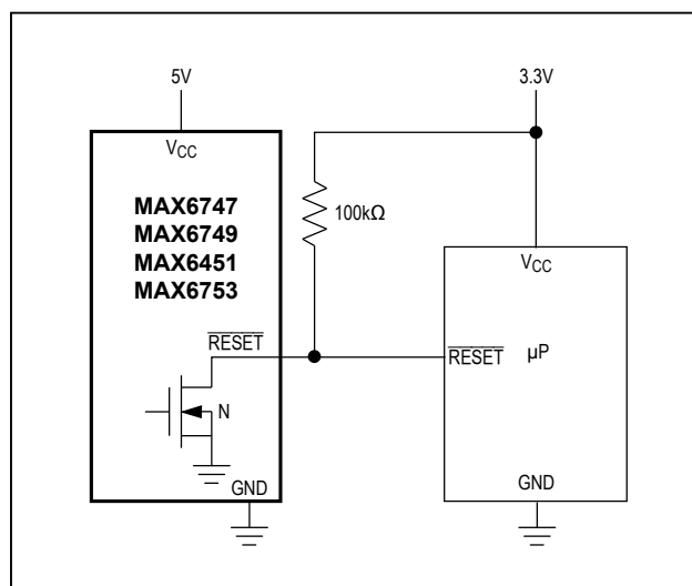
Figure 6. Interfacing to Other Voltage Levels
