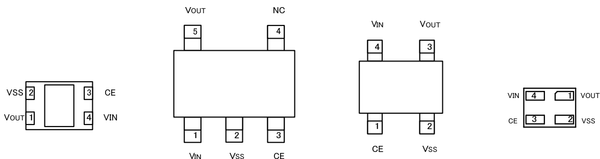
USP-4 (BOTTOM VIEW)
