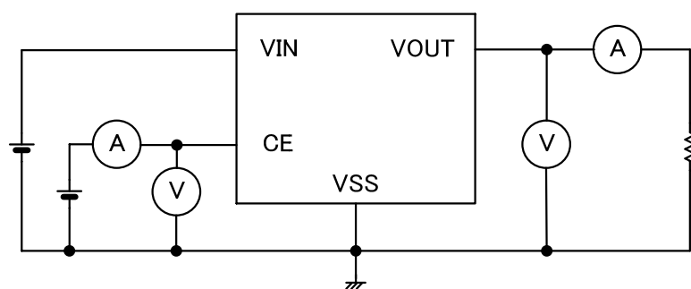
Circuit ③
