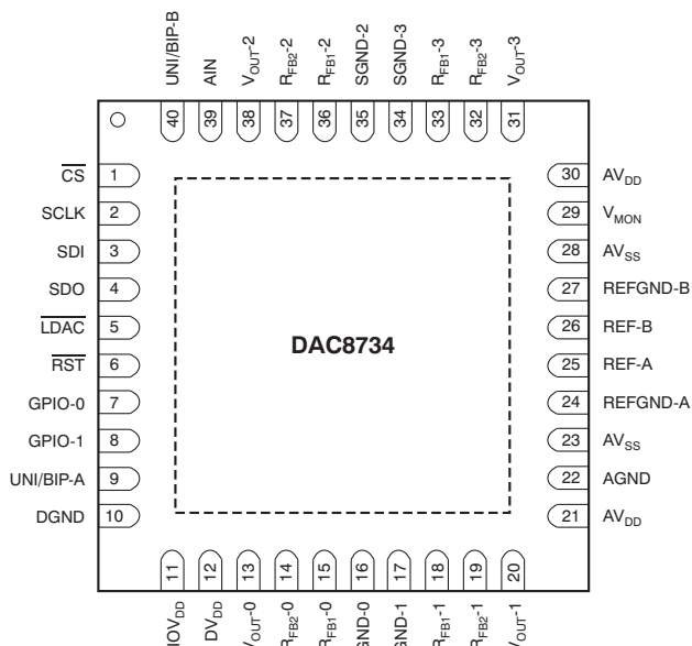
RHA PACKAGE (1) QFN-40 (TOP VIEW)
