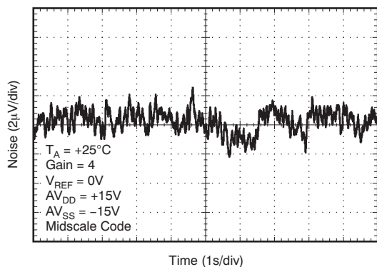
0.1Hz TO 10Hz NOISE (Bipolar Operation)
