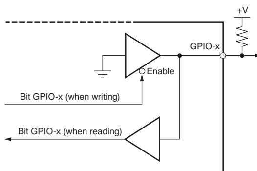
Figure 42. GPIO Pins
