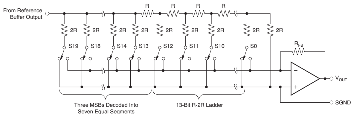
Figure 41. DAC8734 Architecture
