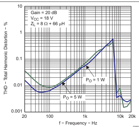
Figure 2. Total Harmonic Distortion vs Frequency (BTL)
