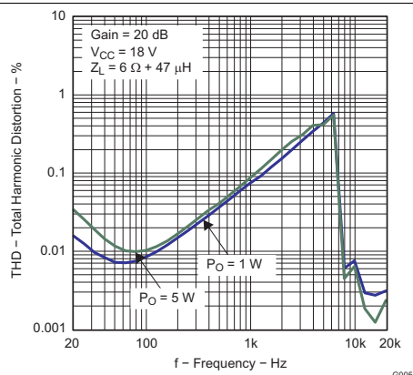
Figure 3. Total Harmonic Distortion vs Frequency (BTL)
