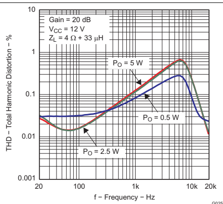
Figure 23. Total Harmonic Distortion vs Frequency (PBTL)
