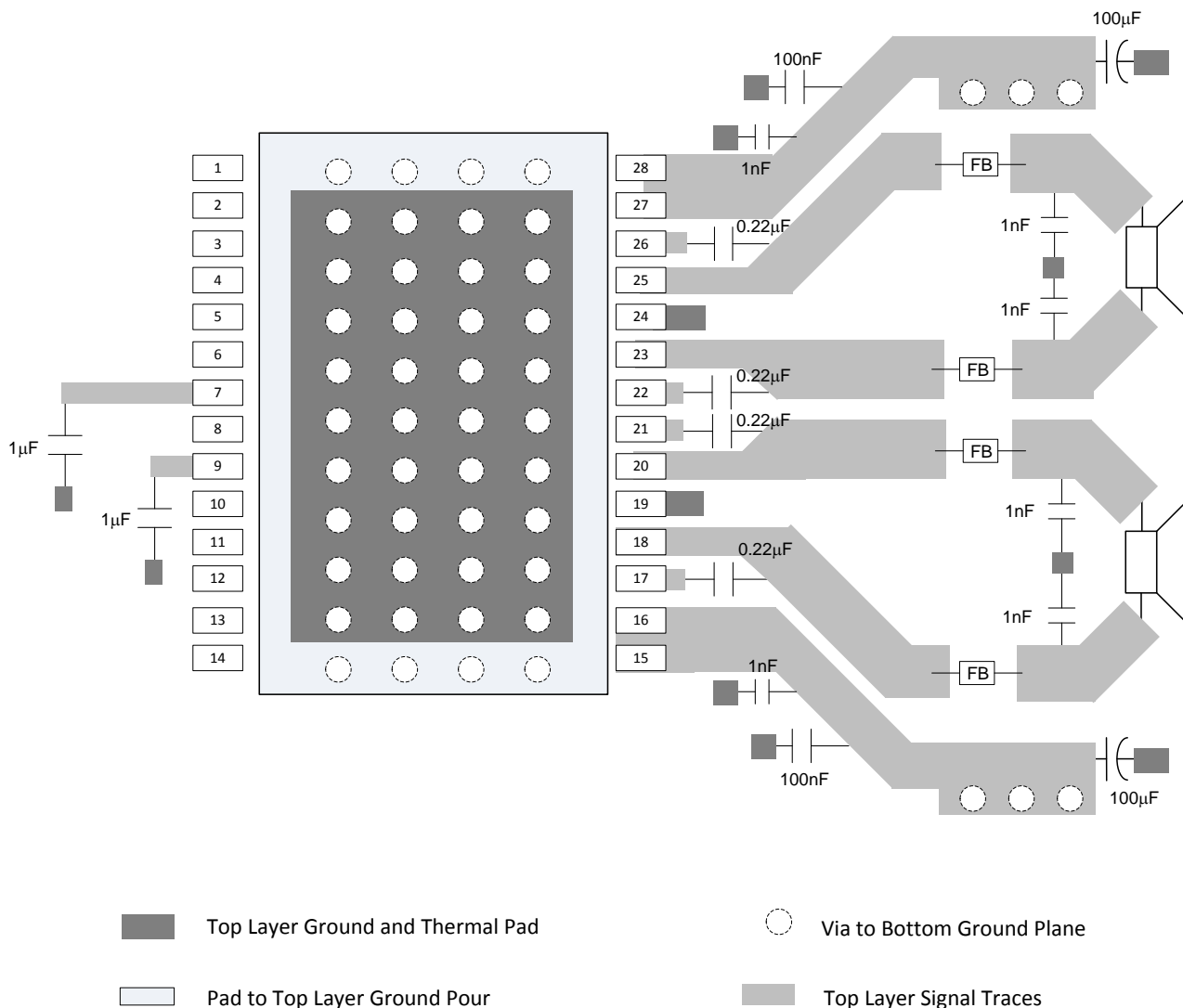
Figure 40. BTL Layout Example
