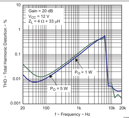
Figure 4. Total Harmonic Distortion vs Frequency (BTL)
