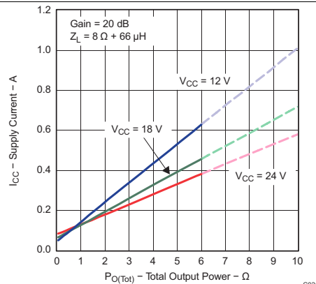
Figure 20. Supply Current vs Total Output Power (BTL)
