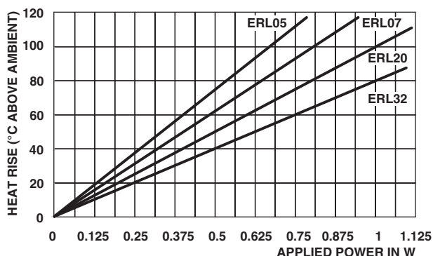
THERMAL RESISTANCE
