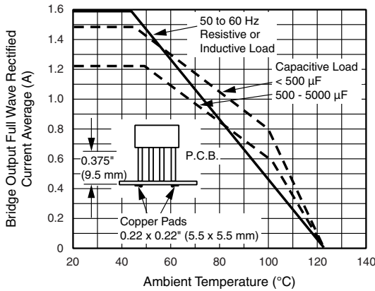
Fig. 1 - Derating Curves Output Rectified Current for B40C1500G...B125C1500G
