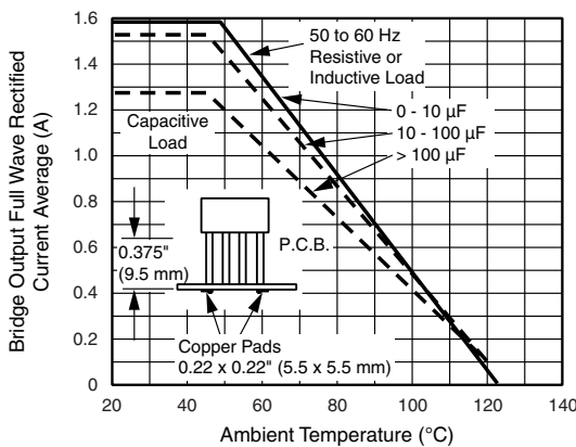
Fig. 2 - Derating Curves Output Rectified Current for B250C1500G...B380C1500G
