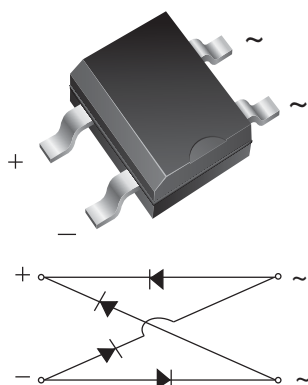
TO-269AA (MBS)
