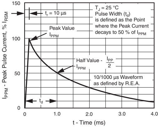
Fig. 3 - Pulse Waveform
