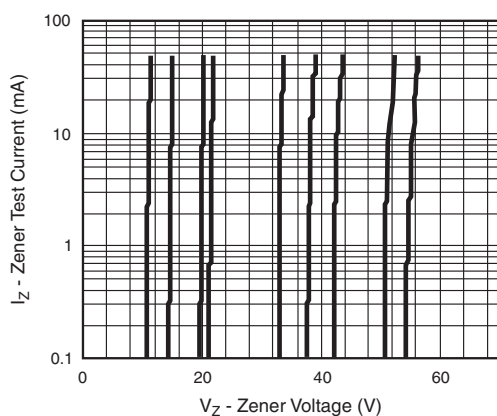
Fig. 5 - Typical Zener Voltage
