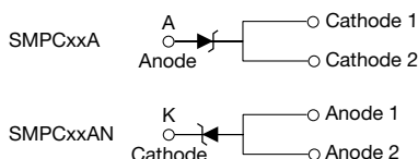
TO-277A (SMPC)
