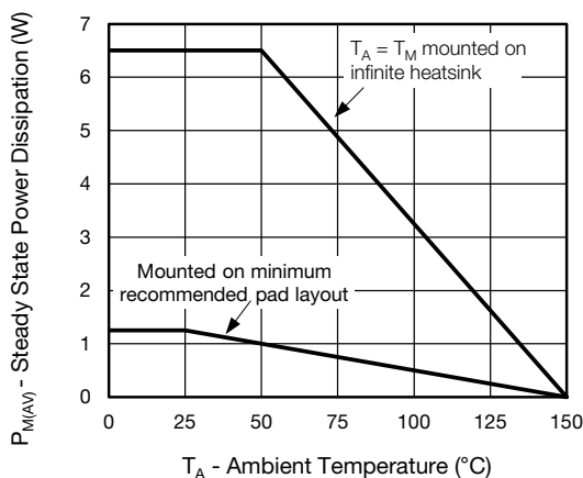
Fig. 5 - Steady State Power Dissipation
