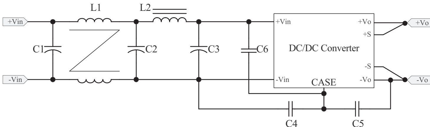
Figure 5 Recommended Circuit for EN55022 Class B
