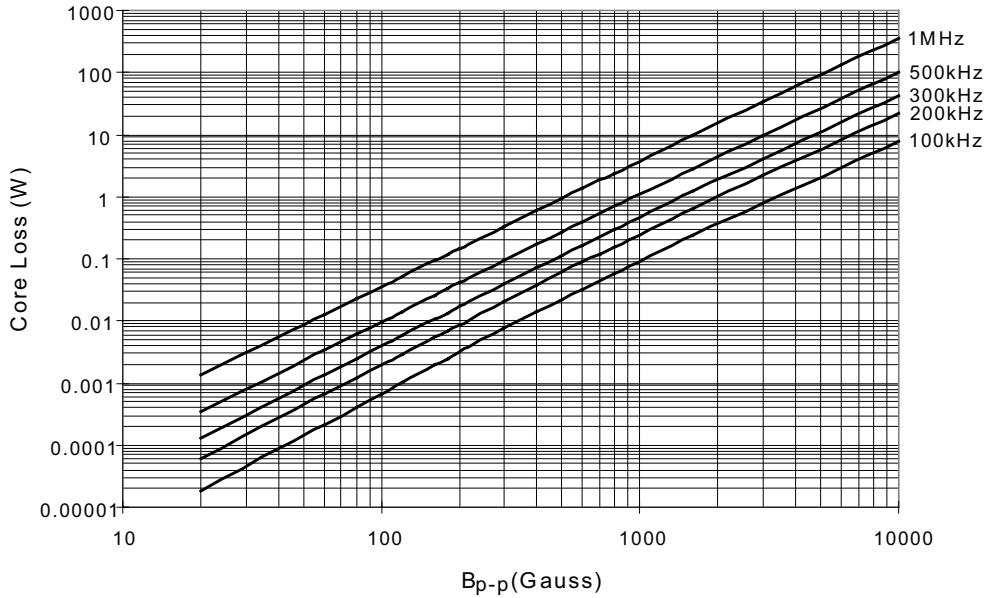
Core Loss vs B_{p-p}
