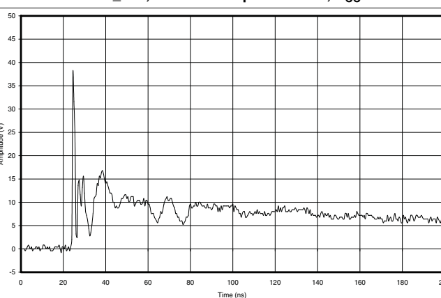
Figure 4. IEC Clamping Waveforms 8-kV Contact, 1-GHz Bandwidth
