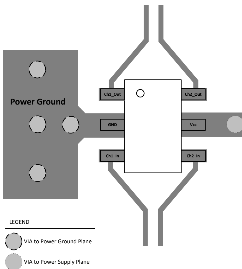
Figure 9. Layout Recommendation
