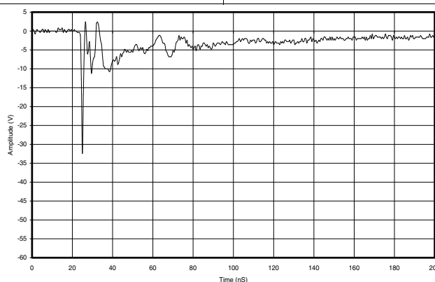
Figure 5. IEC Clamping Waveforms -8-kV Contact, 1-GHz Bandwidth
