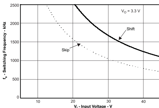
Figure 42. Maximum Switching Frequency vs. Input Voltage
