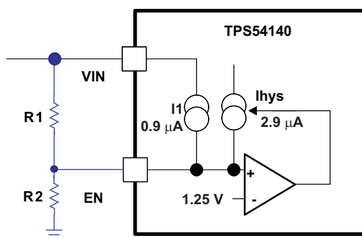
Figure 28. Adjustable Undervoltage Lockout (UVLO)
