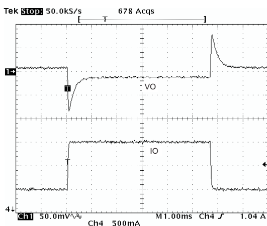
Figure 52. Load Transient
