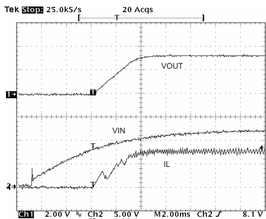
Figure 54. VIN Power Up
