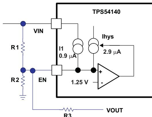
Figure 29. Adding Additional Hysteresis
