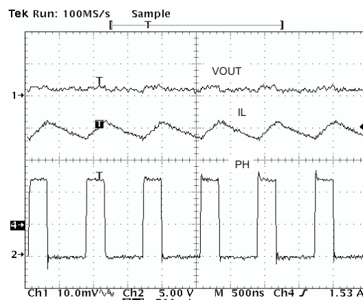
Figure 55. Output Ripple CCM
