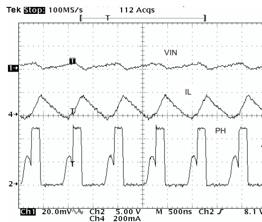
Figure 59. Input Ripple DCM
