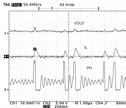
Figure 57. Output Ripple, PSM
