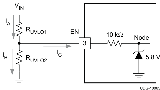
Figure 30. Node Voltage
