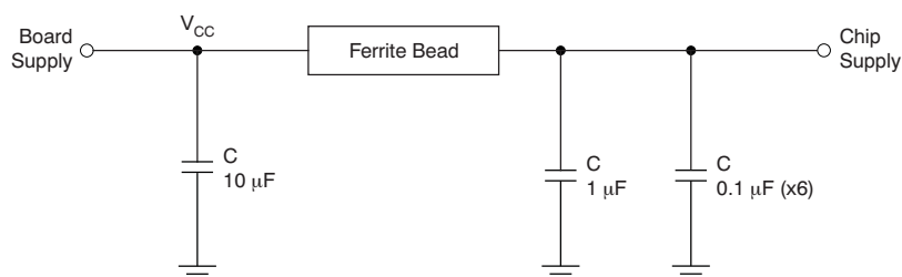
Figure 23. Power-Supply Decoupling
