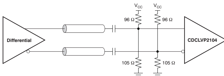
Figure 18. AC-Coupled Differential Inputs to CDCLVP2104 ( V_{CC} = 2.5\text{ V} )
