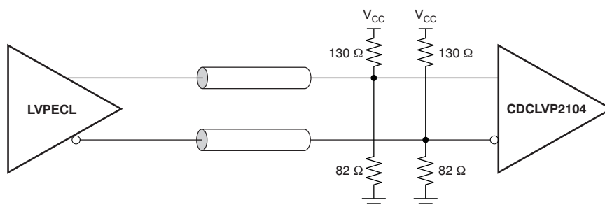
Figure 17. DC-Coupled LVPECL Inputs to CDCLVP2104 ( V_{CC} = 3.3\text{ V} )
