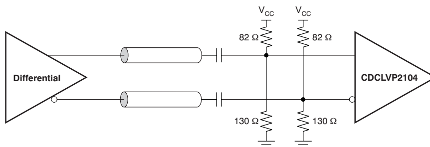
Figure 19. AC-Coupled Differential Inputs to CDCLVP2104 ( V_{CC} = 3.3 \text{ V} )
