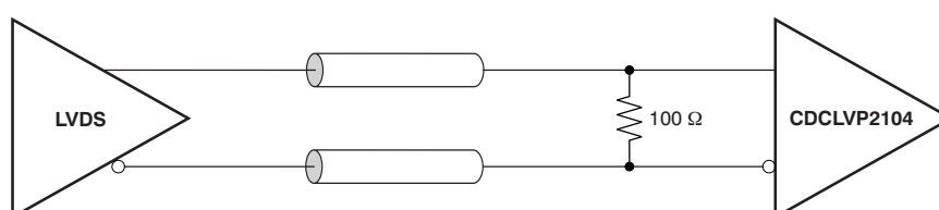
Figure 8. DC-Coupled LVDS Input During Device Test
