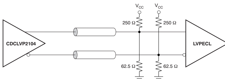
(a) Output DC Termination
