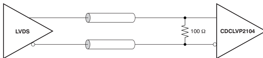
Figure 15. DC-Coupled LVDS Inputs to CDCLVP2104
