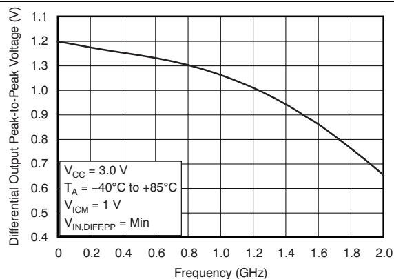
Figure 4. Differential Output Peak-to-Peak Voltage vs Frequency
