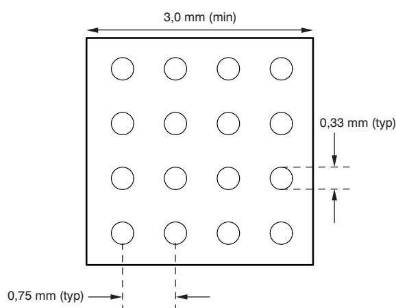
Figure 24. Recommended PCB Layout
