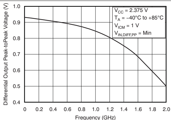
Figure 3. Differential Output Peak-to-Peak Voltage vs Frequency
