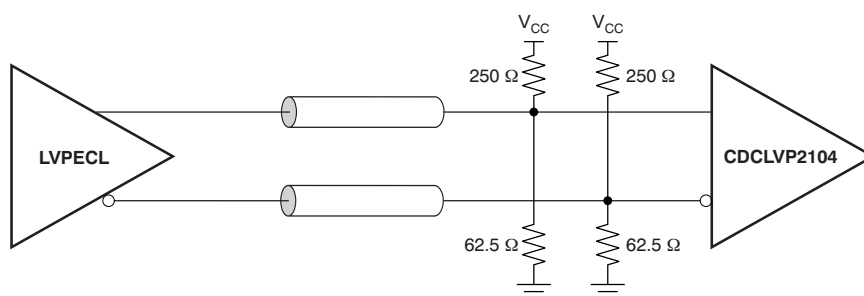
Figure 16. DC-Coupled LVPECL Inputs to CDCLVP2104 ( V_{CC} = 2.5\text{ V} )
