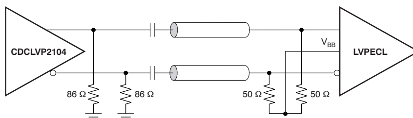
(b) Output AC Termination
