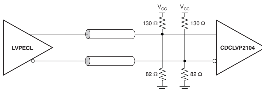
Figure 7. DC-Coupled LVPECL Input During Device Test
