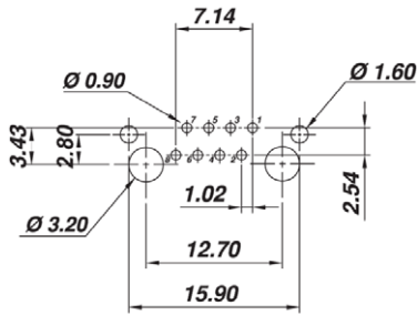
PC Layout (Top View)
