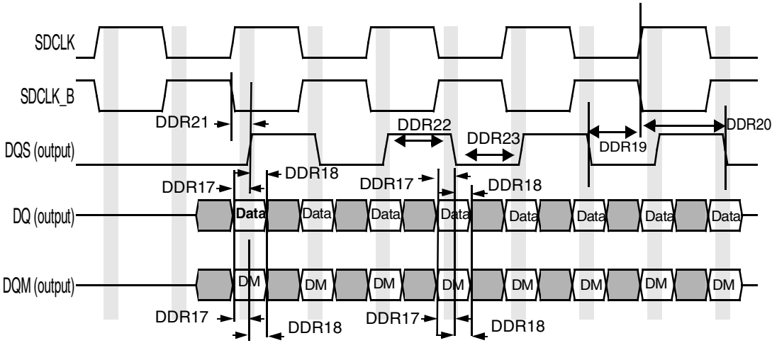
Figure 32. DDR2 SDRAM Write Cycle Timing Diagram
