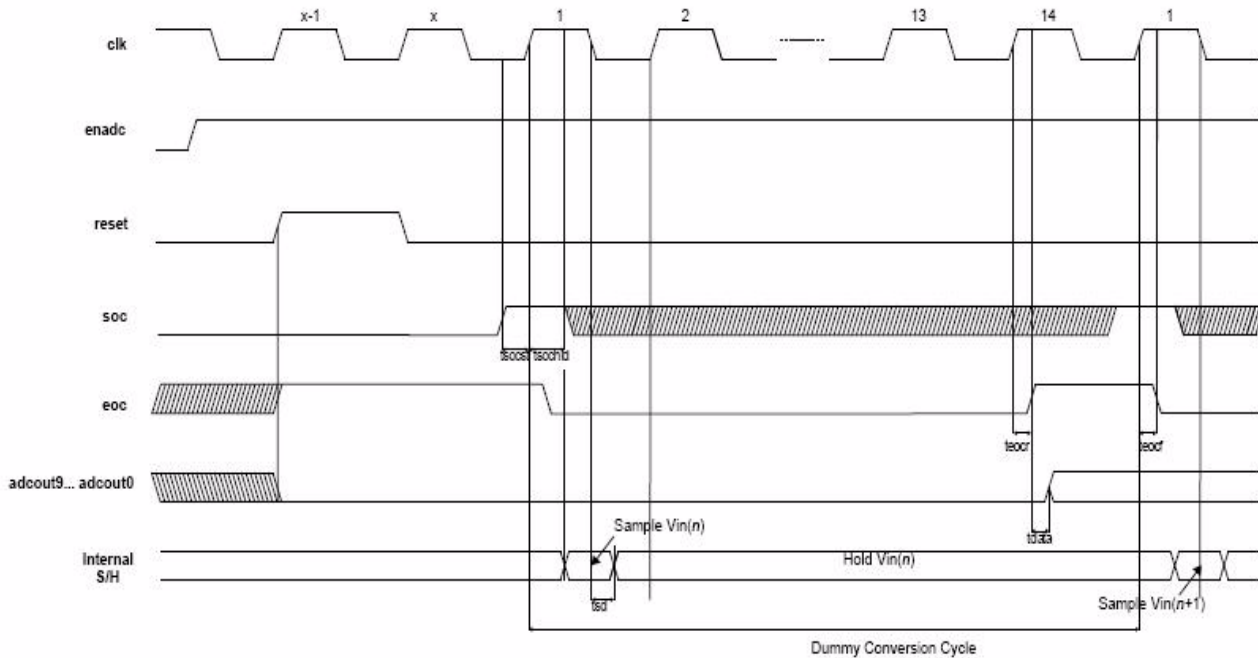
Figure 82. Start-up Sequence
