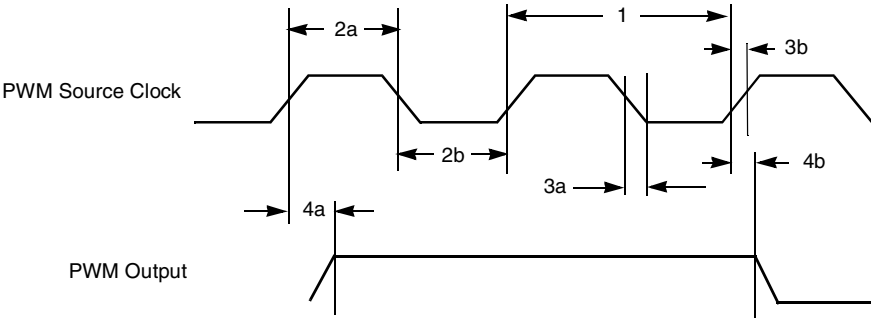
Figure 67. PWM Timing
