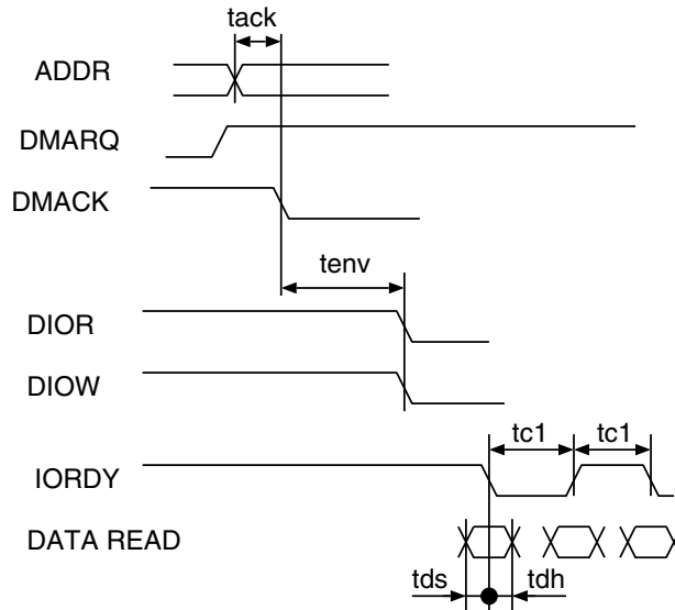
Figure 15. Timing for UDMA In-Transfer Start
