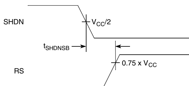
Figure 63. Timing Diagram for FlexCAN Shutdown-to-Standby Signal
