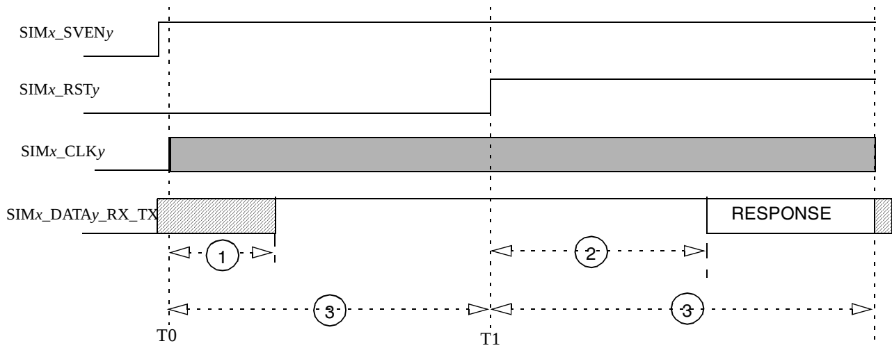
Figure 70. Active-Low-Reset SIM Card Reset Sequence
