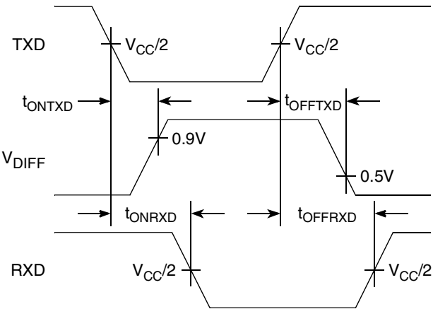
Figure 60. FlexCAN Timing Diagram
