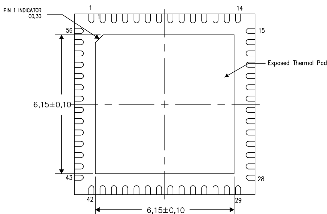
Bottom View
