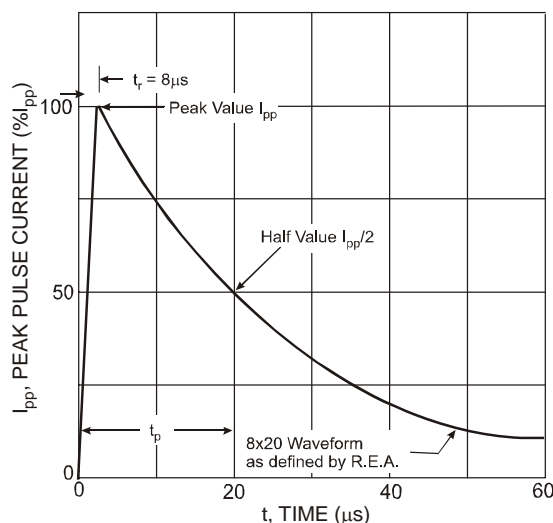
Fig. 2 Pulse Waveform
