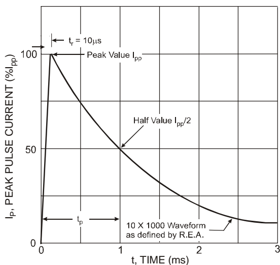
Fig. 1 Pulse Waveform
