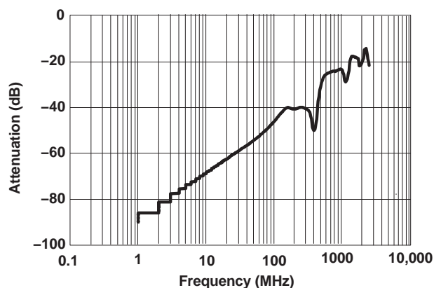
Figure 2. OFF Isolation vs Frequency
