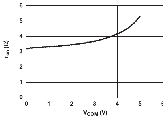
Figure 4. r_{ON} ( \Omega ) vs V_{COM} (V)
