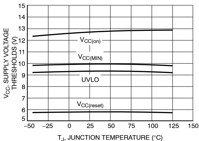
Figure 3. Supply Voltage Thresholds vs. Junction Temperature
