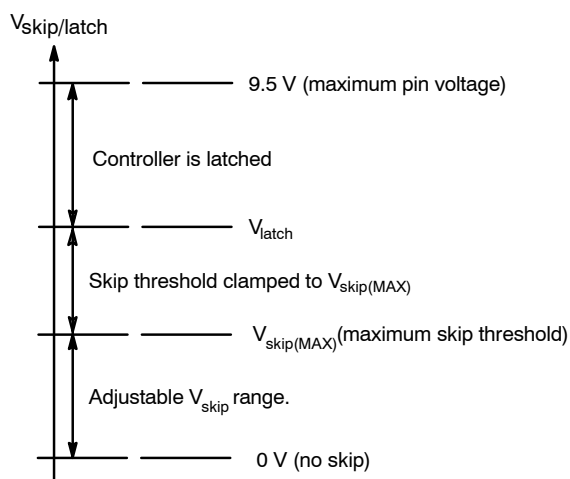
Figure 39. NCP1218 VSkip/latch Pin Operating Regions
