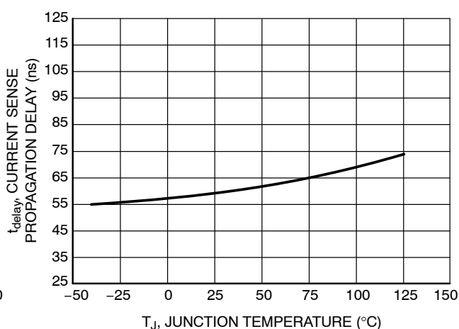
Figure 14. Current Sense Propagation Delay vs. Junction Temperature
