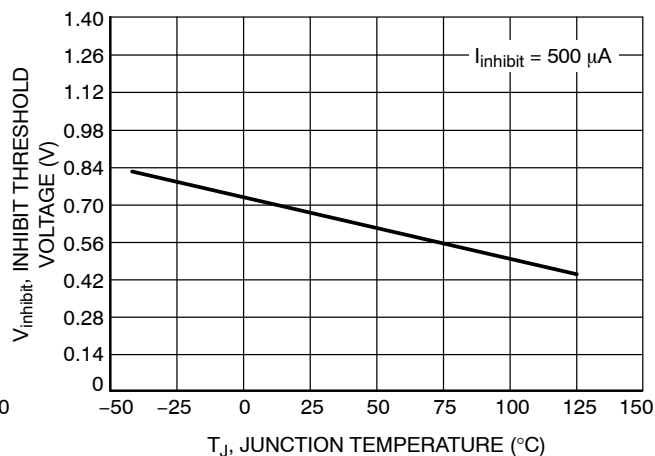
Figure 4. Inhibit Threshold Voltage vs. Junction Temperature
