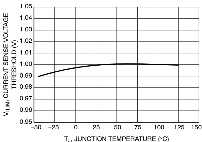
Figure 12. Current Sense Voltage Threshold vs. Junction Temperature
