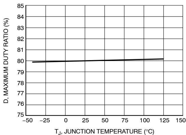
Figure 16. Maximum Duty Ratio vs. Junction Temperature
