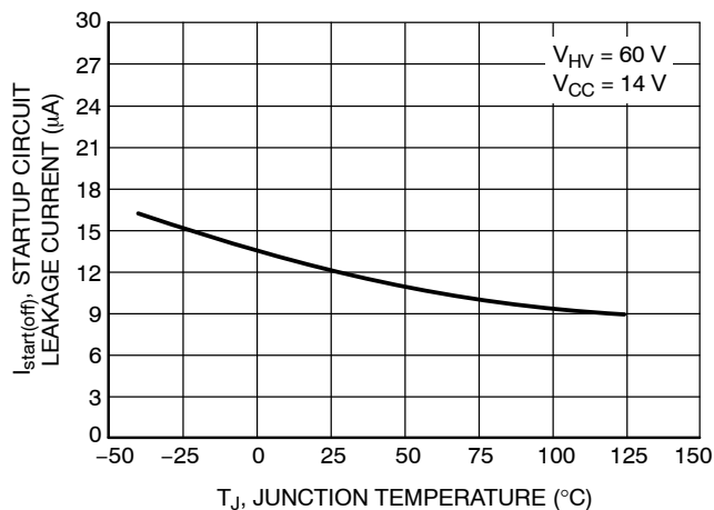
Figure 8. Startup Circuit Leakage Current vs. Junction Temperature
