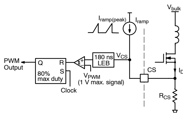
Figure 30. Current-Mode Implementation
