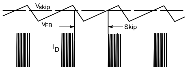
Figure 37. Skip Operation
