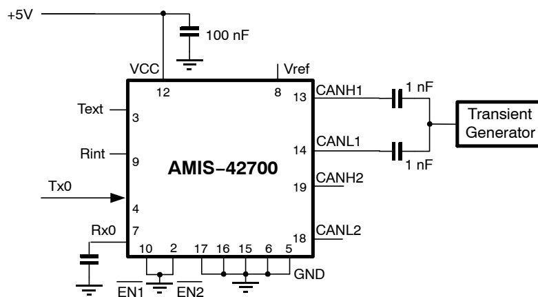
Figure 5. Test Circuit for Automotive Transients
