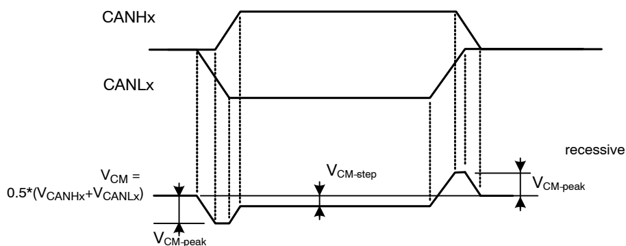
Figure 10. Common-mode Voltage Peaks (see measurement set-up Figure 9)
