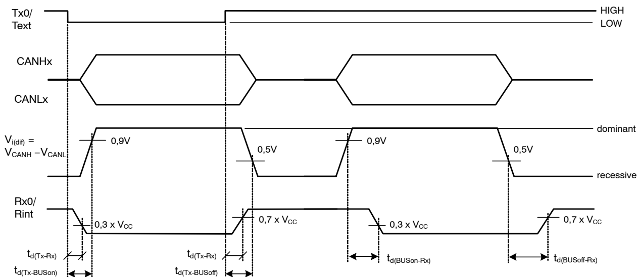
Figure 8. Timing Diagram for AC Characteristics
