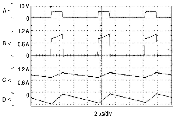
Figure 14. Switching Waveforms
