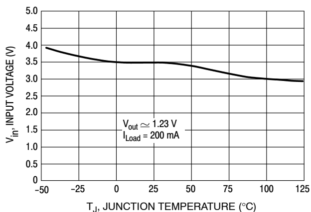
Figure 11. Minimum Supply Operating Voltage
