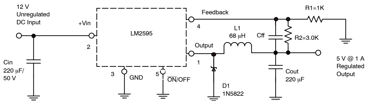
Figure 1. Typical Application
