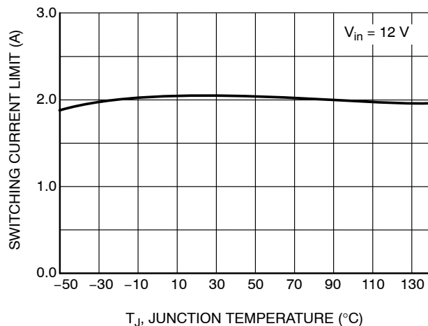
Figure 6. Current Limit
