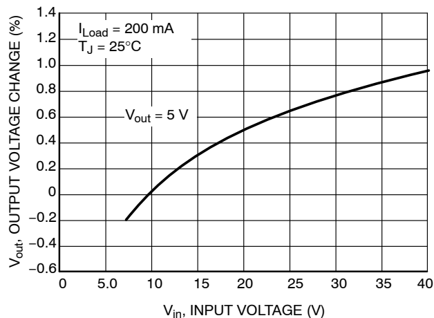
Figure 4. Line Regulation
