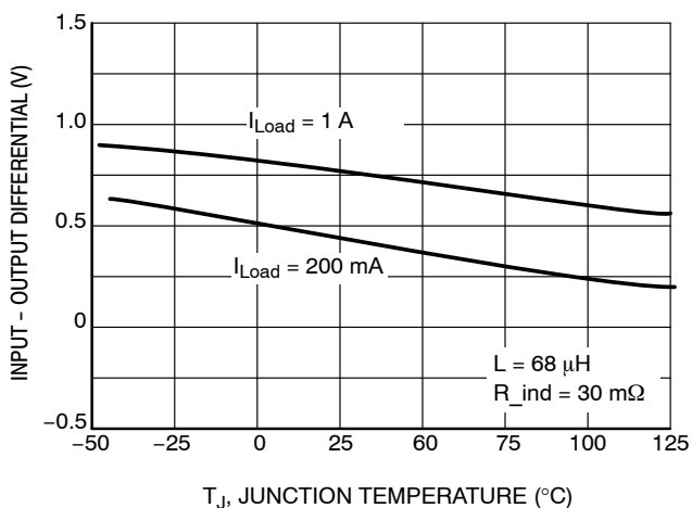
Figure 5. Dropout Voltage
