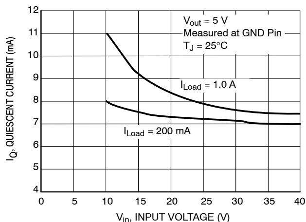
Figure 7. Quiescent Current
