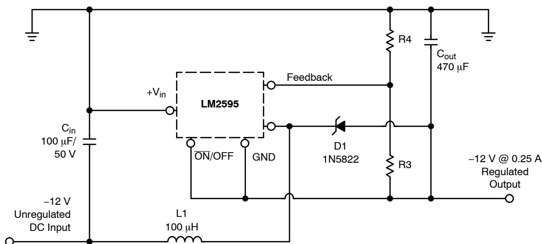
Figure 27. Negative Boost Regulator
