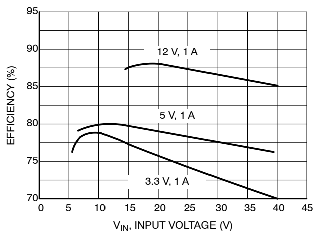
Figure 13. Efficiency
