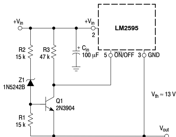
Figure 30. Undervoltage Lockout Circuit for Buck-Boost Converter
