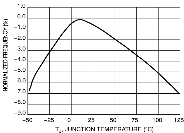
Figure 10. Switching Frequency
