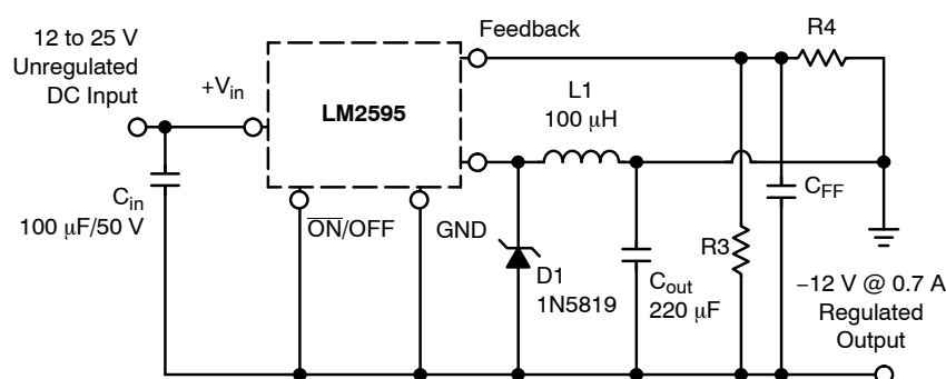
Figure 23. Inverting Buck–Boost Develops –12 V
