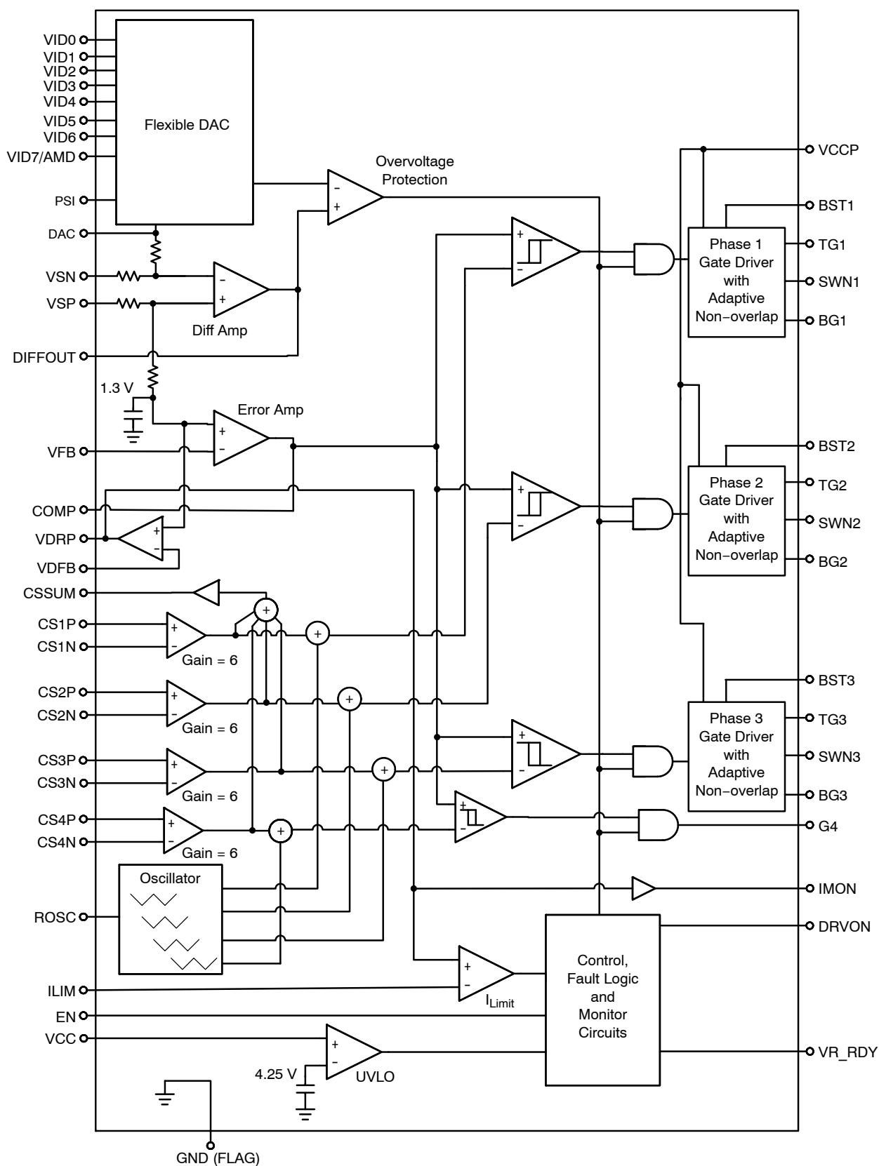
Figure 1. NCP5395 Functional Block Diagram
