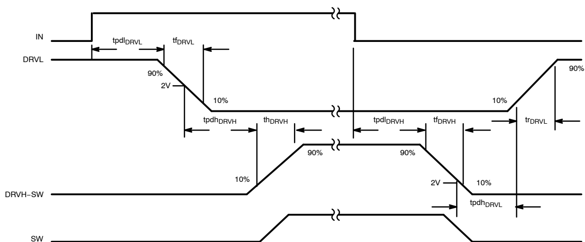
Figure 5. Timing Diagram
