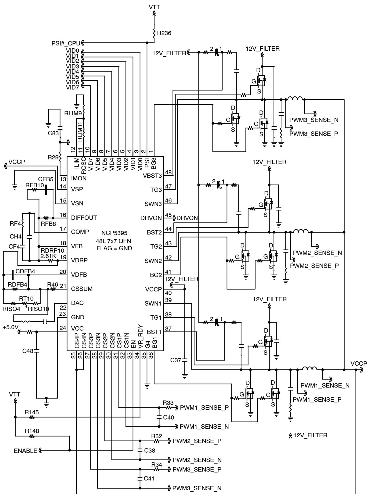
Figure 3. Typical 3 Phase Application
