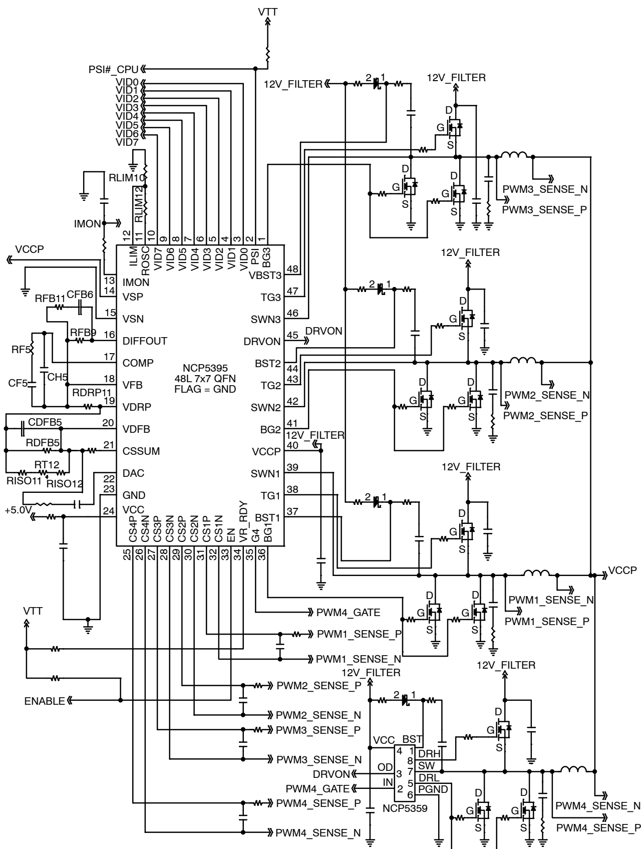
Figure 4. Typical 4 Phase Application
