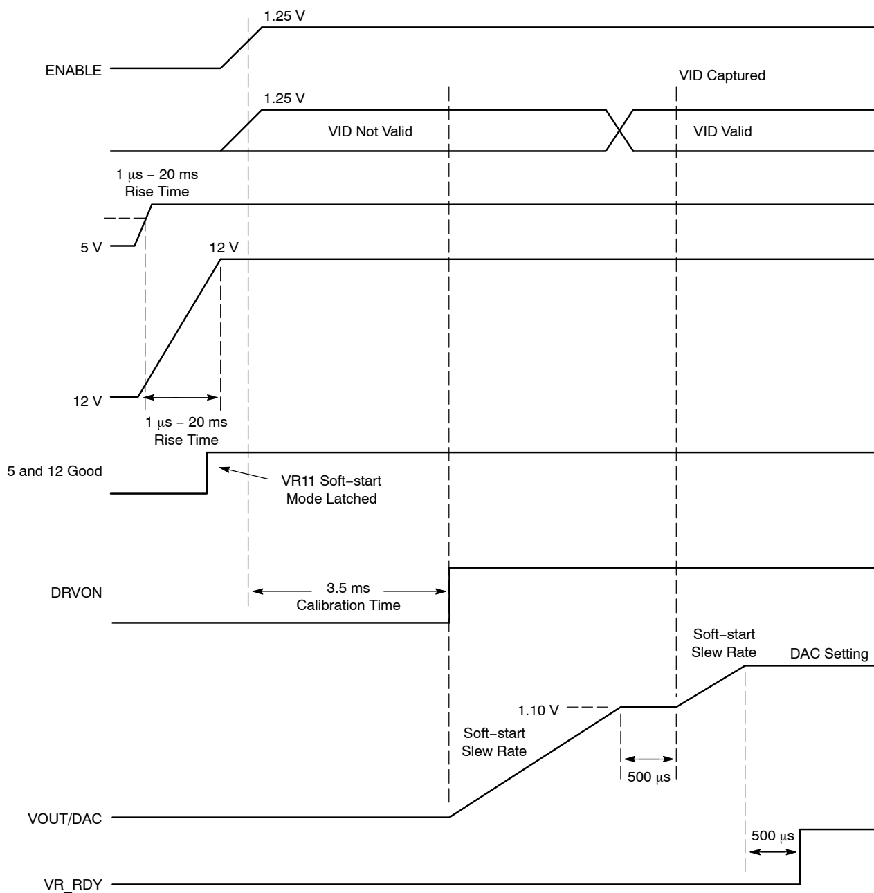
Figure 6. VR11.1 Start Up Timing Diagram
