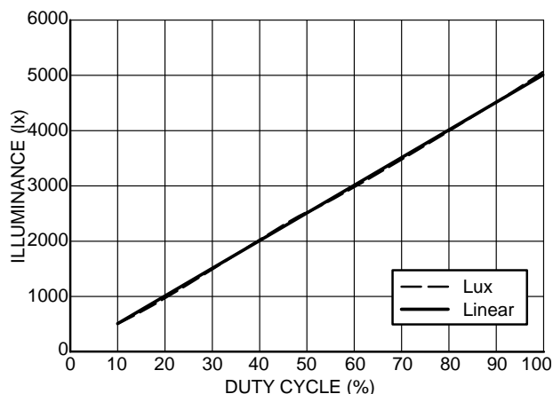
Figure 13. Luminous Emittance vs. Duty Cycle
