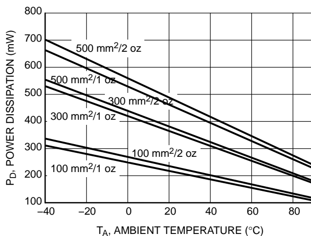
Figure 6. Power Dissipation vs. Ambient Temperature @ T_J = 150^{\circ}\text{C}
