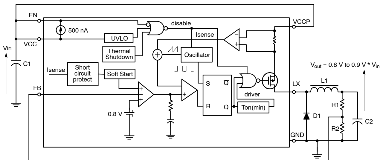
Figure 2. Detail Block Diagram
