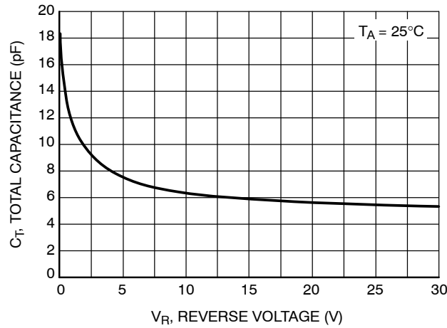
Figure 3. Total Capacitance
