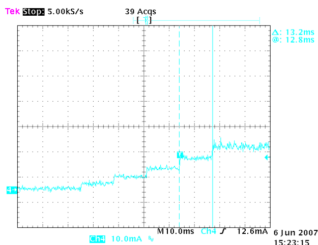
Figure 10. Typical Gradual Dimming UPWARD
