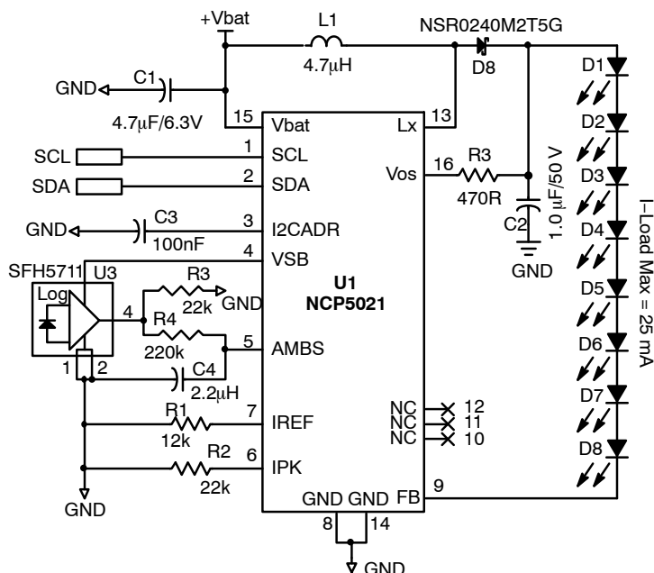
Figure 1. Typical Large Display LED Driver
