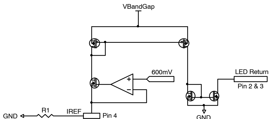
Figure 8. Basic Reference Current Source
