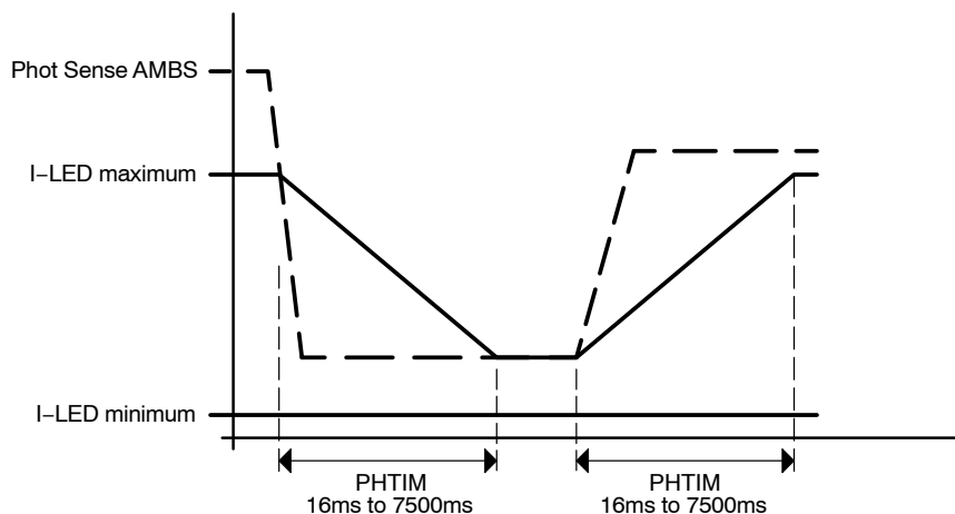
Figure 13. Basic Photo Sense Timing
