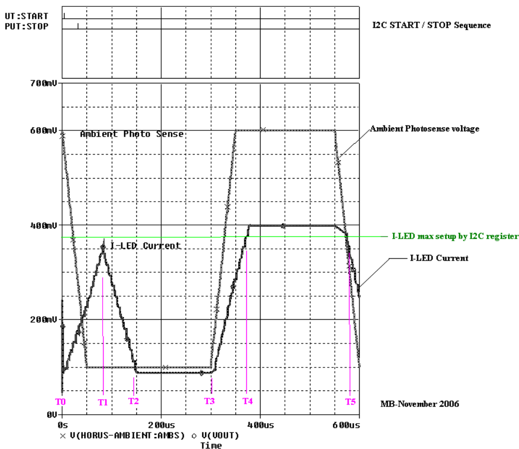
Figure 15. Basic Ambient Photo Sense Regulation (PSpice Simulation)
