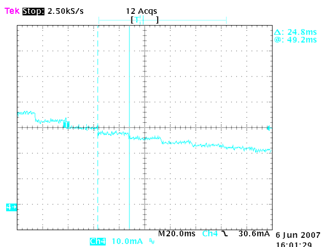
Figure 11. Typical Gradual Dimming DOWNWARD
