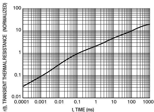
Figure 4. Thermal Response
