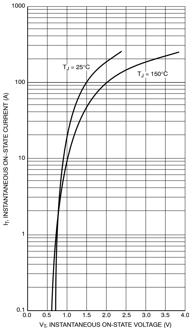
Figure 3. On-State Characteristics
