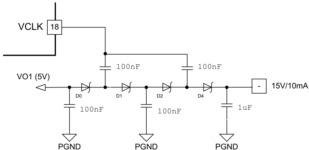
Figure 39. 15-V / 10-mA Charge Pump Configuration
