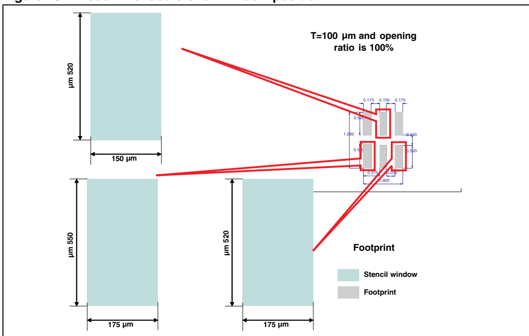
Figure 18. Recommended stencil window position
