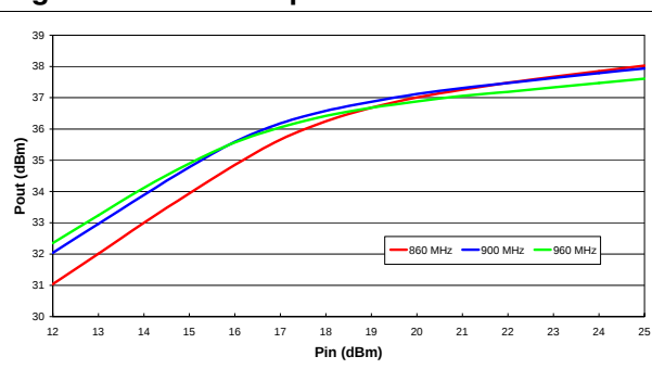
Figure 17. Pout vs. pin 13.6 V / 200 mA
