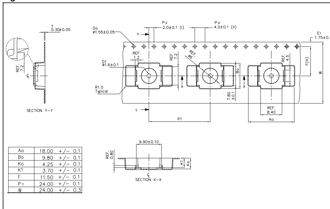
Figure 22. Reel information
