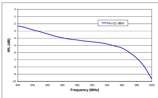
Figure 14. Input return loss vs. frequency 13.6 V / 200 mA
