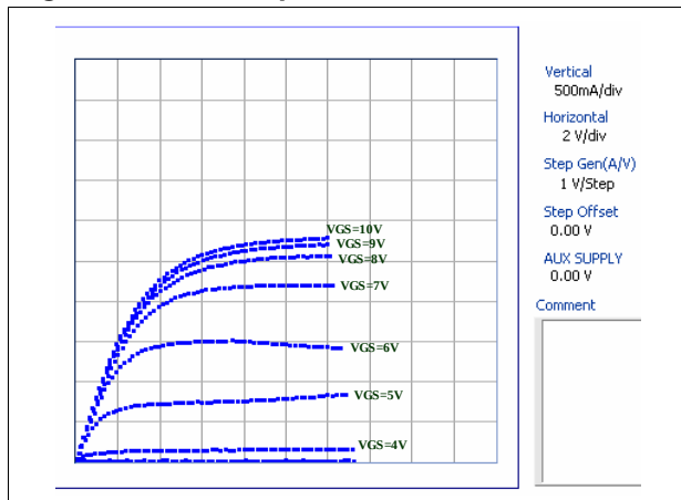
Figure 9. DC output characteristics
