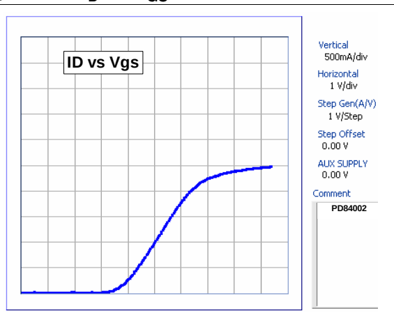
Figure 10. ID vs. VGS
