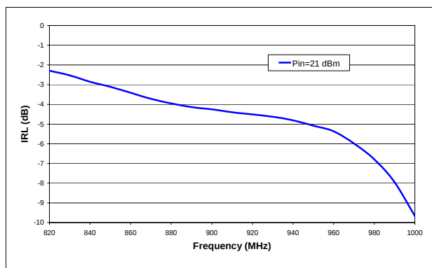
Figure 5. Input return loss vs. frequency 13.6 V / 200 mA
