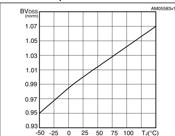
Figure 17. Normalized BV DSS @ 1 mA vs temperature
