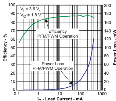
Figure 2. Efficiency vs. Load Current
