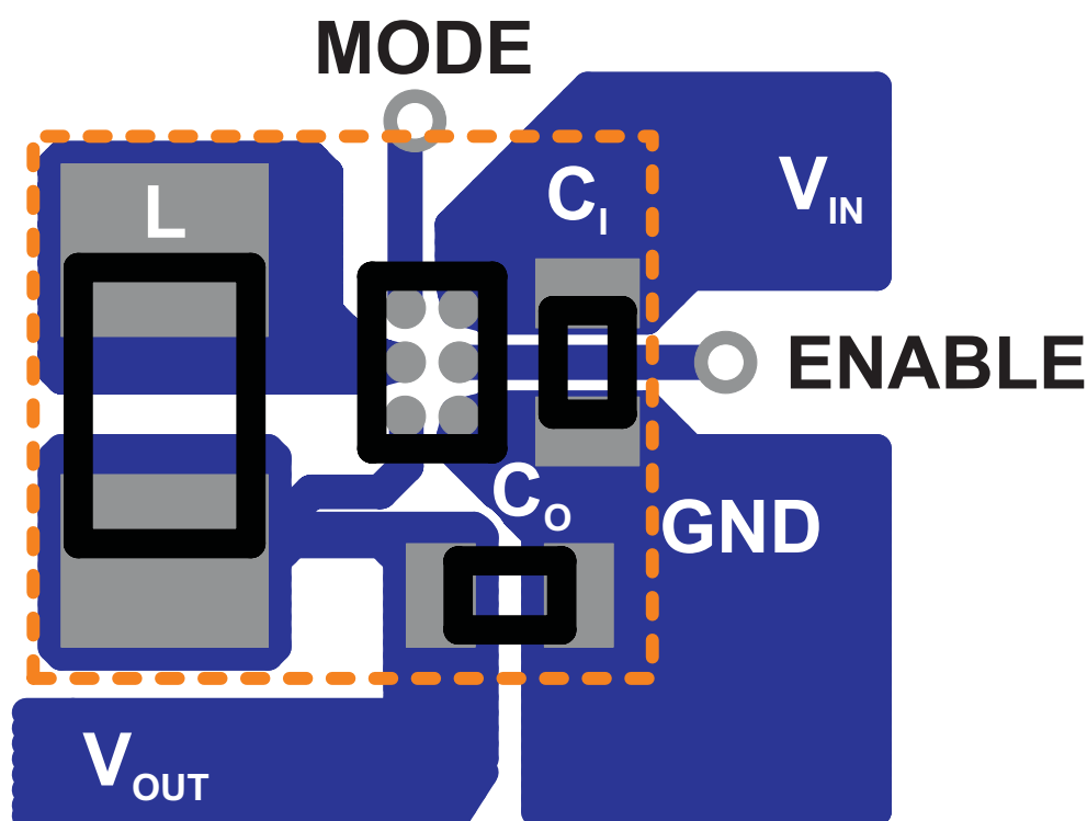
Figure 36. Suggested Layout (Top)
