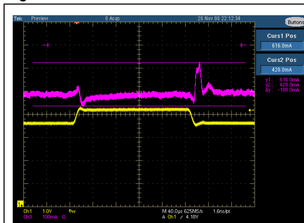
Figure 14. Line transient
