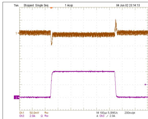
Figure 15. Load Transient Response
