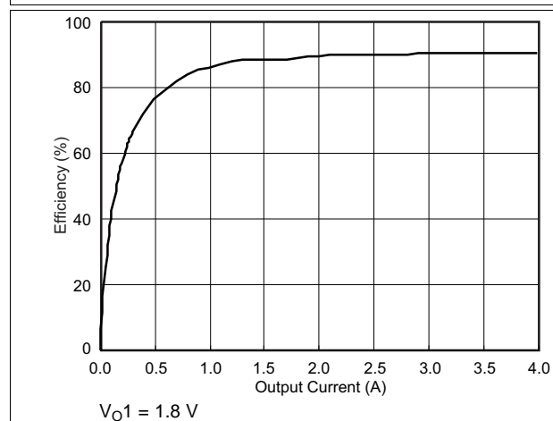
Figure 19. 1.8-V Efficiency vs Output Current (CH1)
