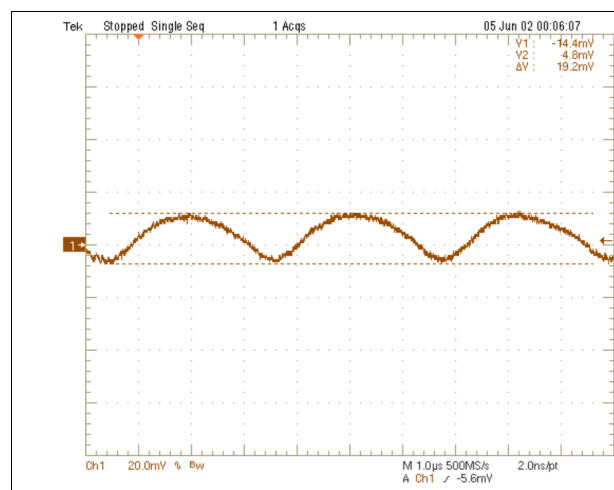
Figure 21. 1.8-V Output Ripple Voltage
