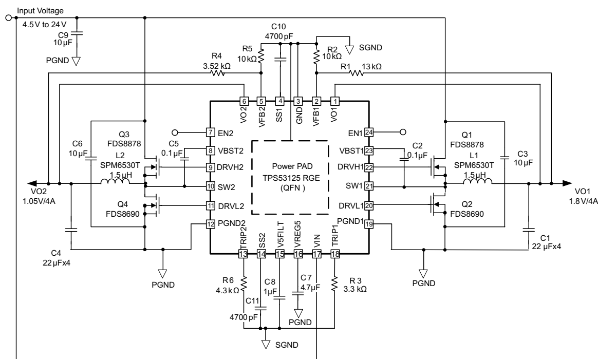
Figure 6. TPS53125 Typical Application Circuit (QFN)
