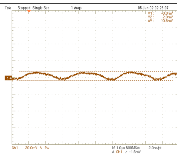
Figure 22. 1.05-V Output Ripple Voltage
