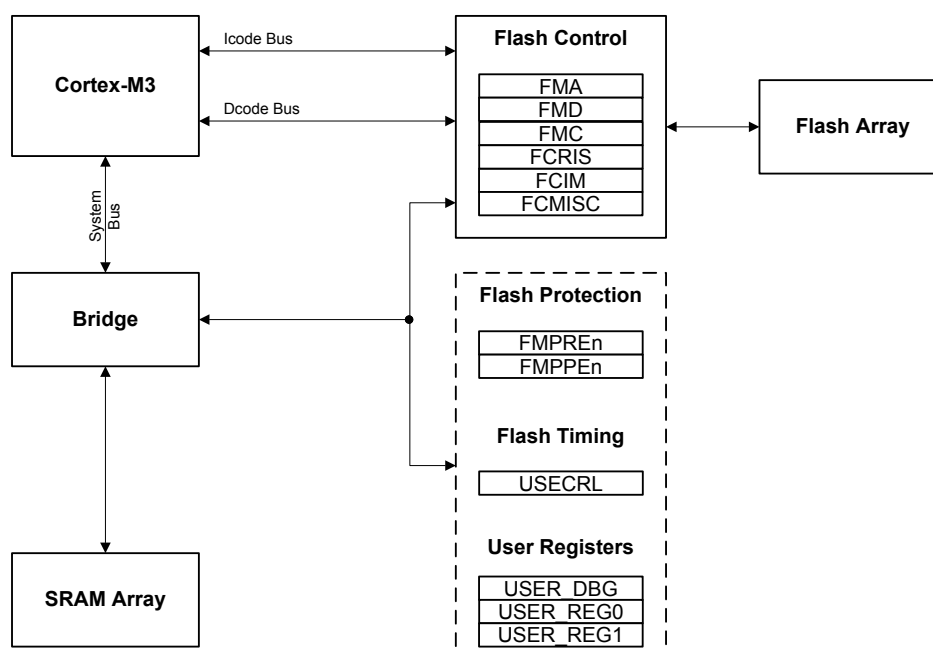
Figure 7-1. Flash Block Diagram
