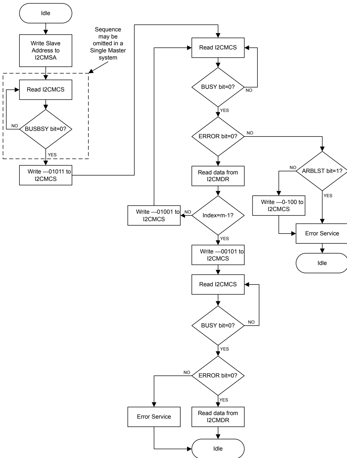
Figure 14-10. Master Burst RECEIVE
