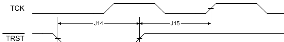
Figure 19-4. JTAG TRST Timing
