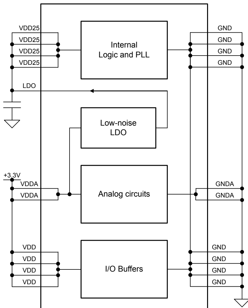
Figure 5-4. Power Architecture
