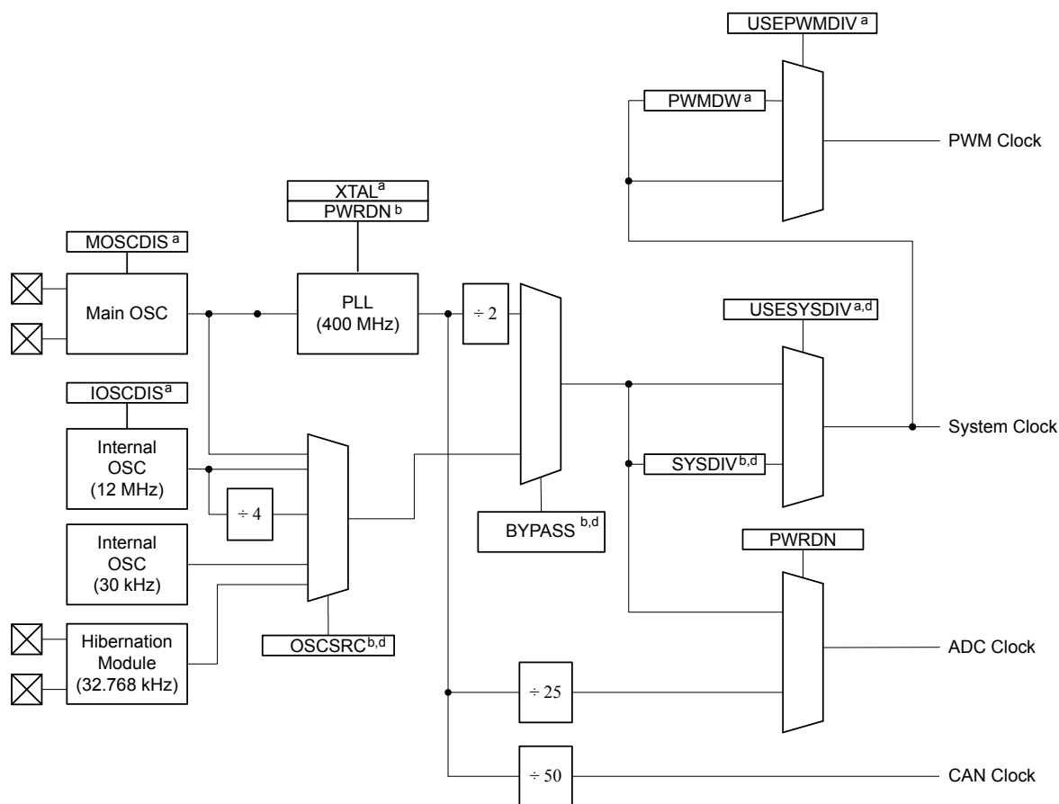
Figure 5-5. Main Clock Tree
