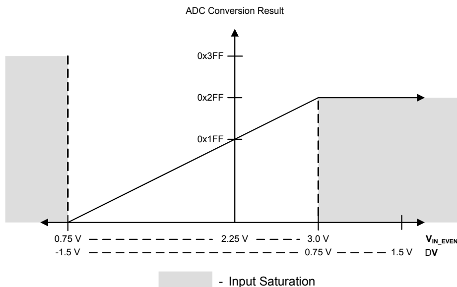
Figure 11-4. Differential Sampling Range, V_{IN\_ODD} = 2.25\text{ V}
