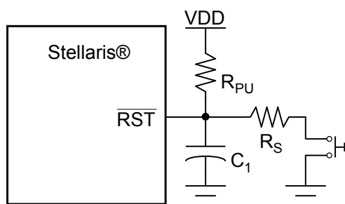
Figure 5-3. Reset Circuit Controlled by Switch
