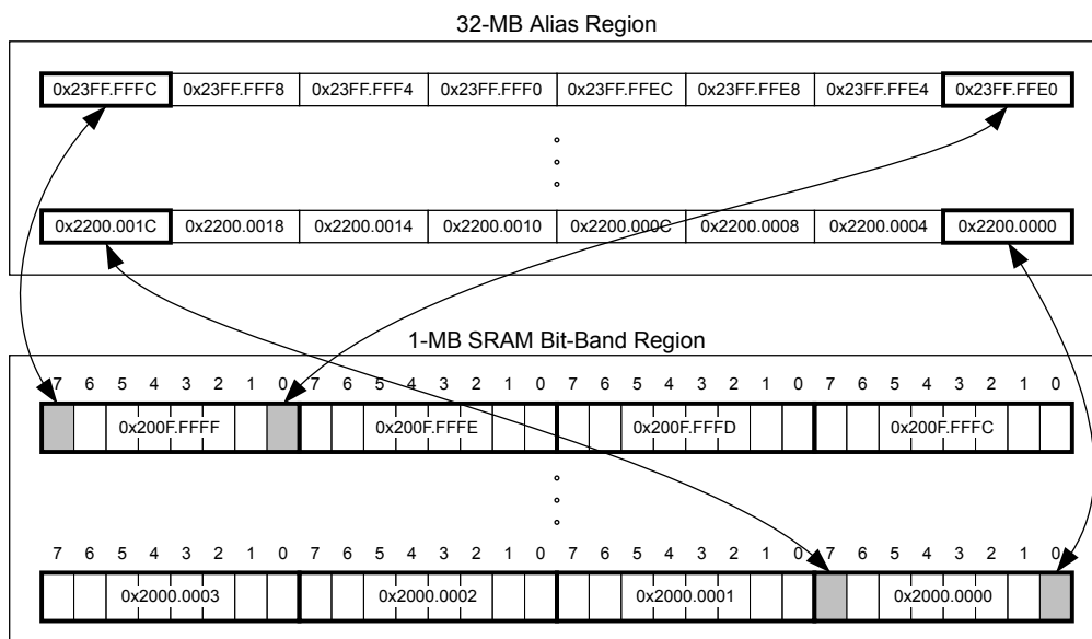
Figure 2-4. Bit-Band Mapping
