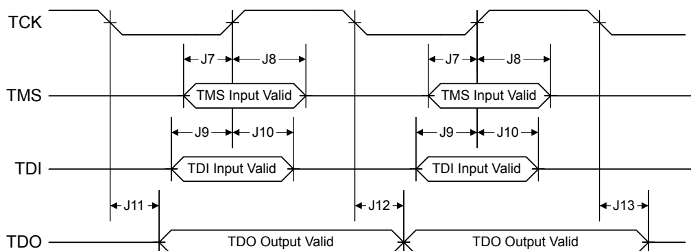
Figure 19-3. JTAG Test Access Port (TAP) Timing
