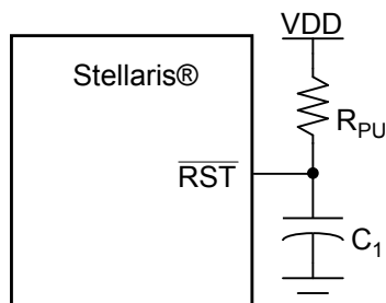
Figure 5-2. External Circuitry to Extend Power-On Reset
