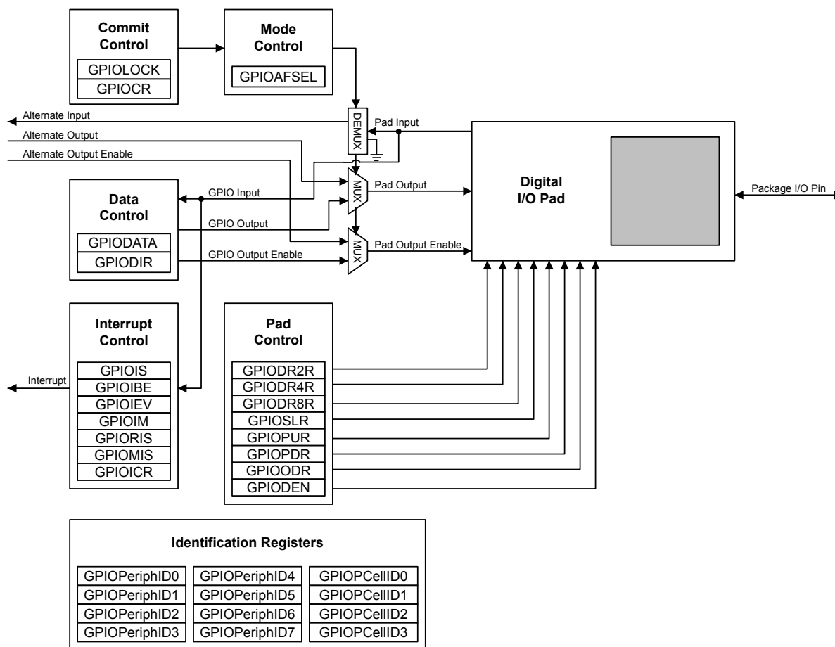
Figure 8-1. GPIO Port Block Diagram
