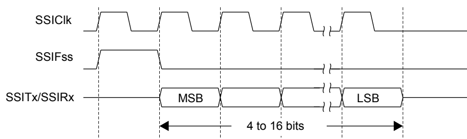
Figure 13-2. TI Synchronous Serial Frame Format (Single Transfer)
