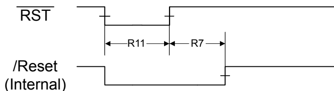
Figure 19-6. Power-On Reset Timing
