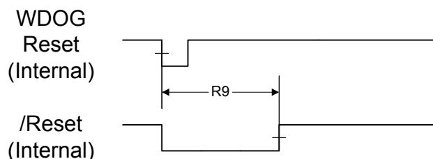
Figure 19-9. Watchdog Reset Timing
