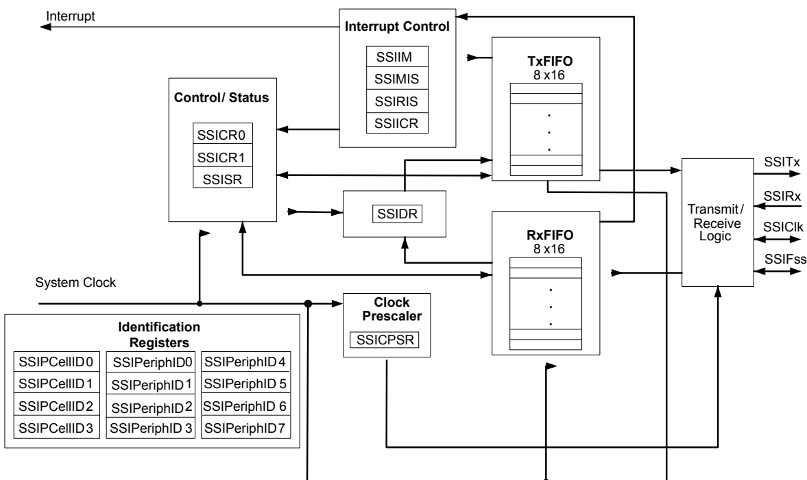
Figure 13-1. SSI Module Block Diagram
