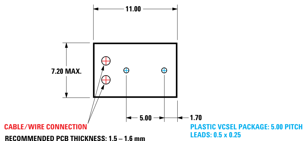
Figure 2. Suggested ADVN-6340 PCB mounting guide
