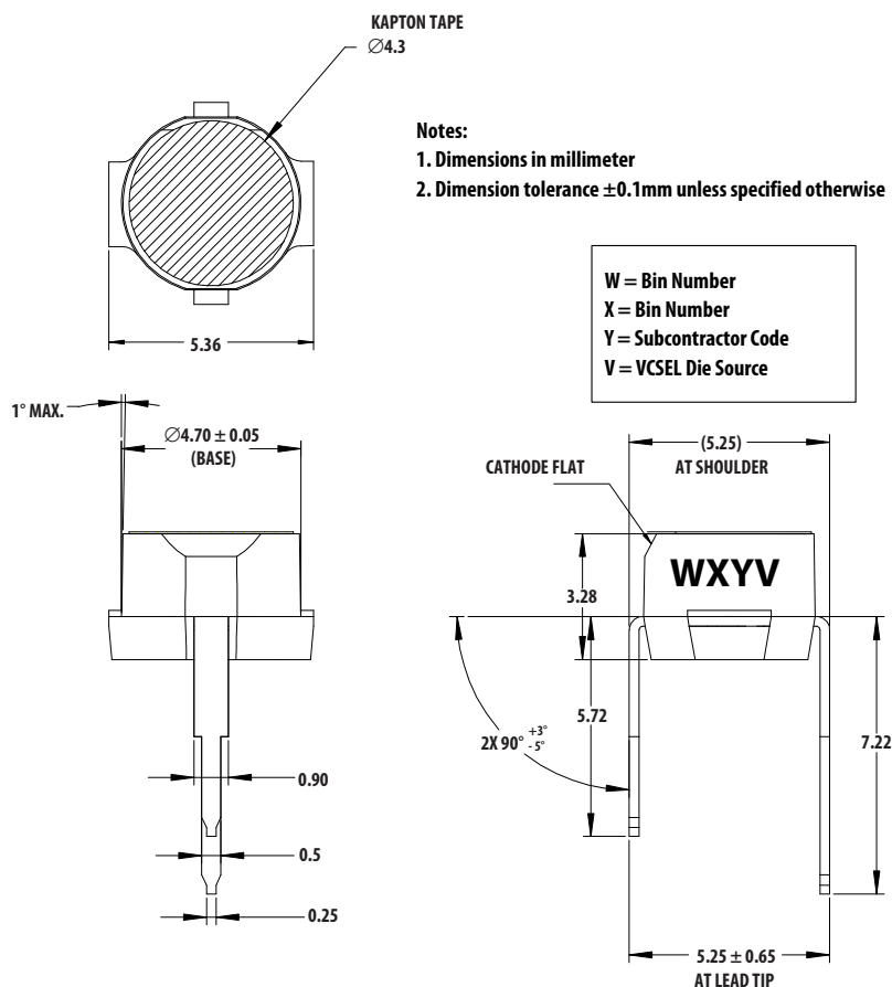
Figure 1. Outline drawing for ADVN-6340 VCSEL
