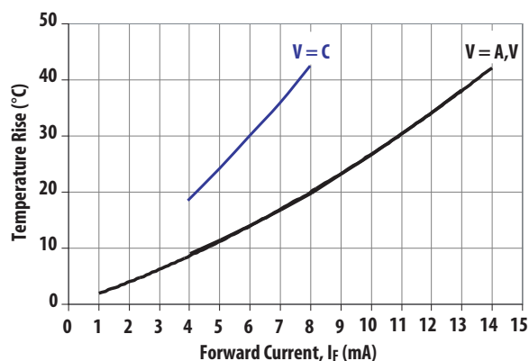
Figure 5. Junction temperature rise vs. forward current
