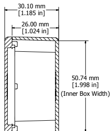
SECTION B-B End View of Assembly
