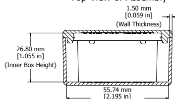
SECTION A-A Side View of Assembly
