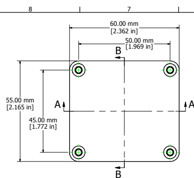
Top View of Assembly
