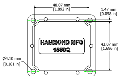
View Looking Inside Lid
