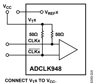
Figure 19. DC-Coupled CML Input Termination
