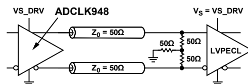
Figure 16. DC-Coupled, 3.3 V LVPECL Y-Termination
