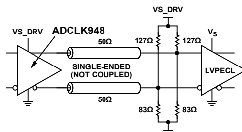
Figure 15. DC-Coupled, 3.3 V LVPECL Far-End Thevenin Termination
