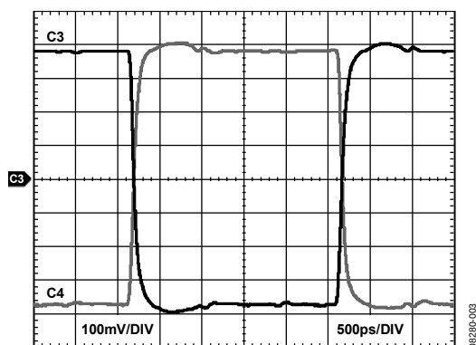
Figure 3. LVPECL Output Waveform @ 200 MHz
