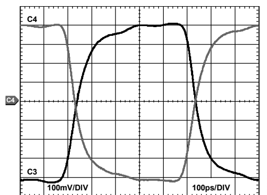
Figure 6. LVPECL Output Waveform @ 1000 MHz
