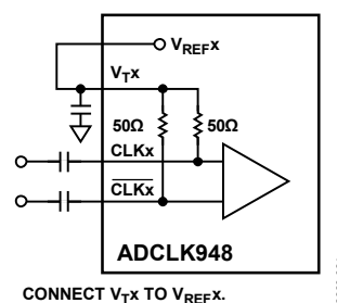
Figure 21. AC-Coupled Input Termination, Such as LVDS and LEVPECL
