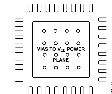
Figure 18. PCB Land for Attaching Exposed Paddle
