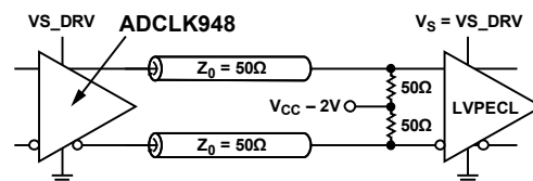
Figure 14. DC-Coupled, 3.3 V LVPECL
