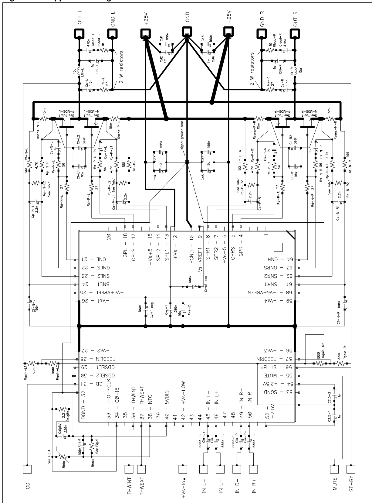
Figure 3. Application diagrams
