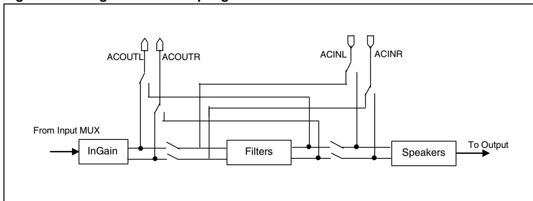
Figure 21. Diagram of AC coupling
