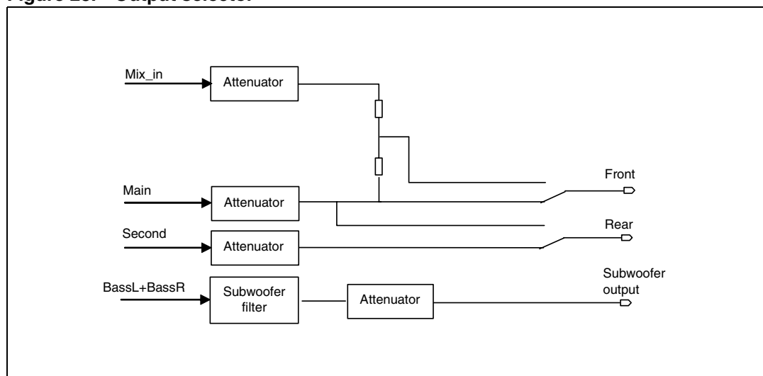
Figure 23. Output selector
