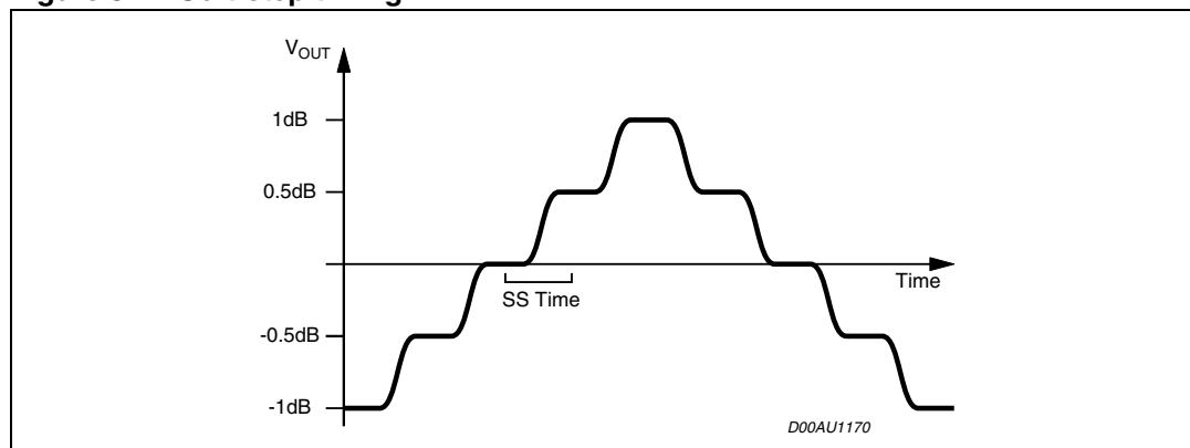
Figure 8. Soft-step timing
