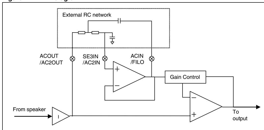
Figure 22. HPF diagram
