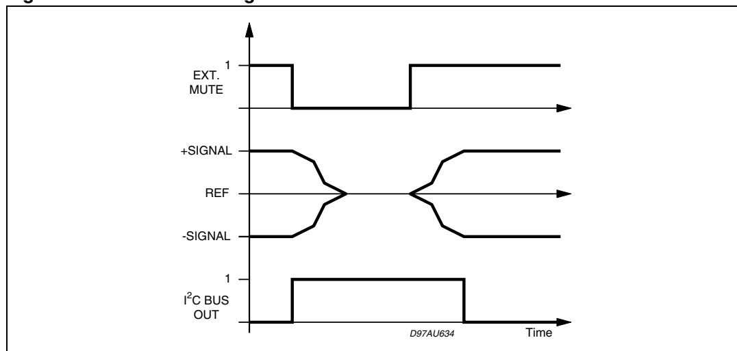
Figure 7. Soft-mute timing
