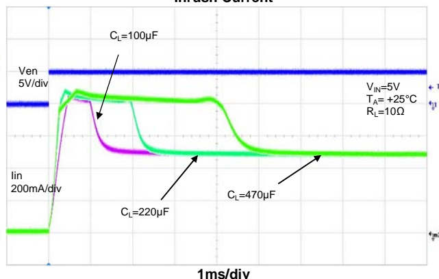
Inrush Current
