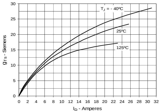
Fig. 8. Transconductance
